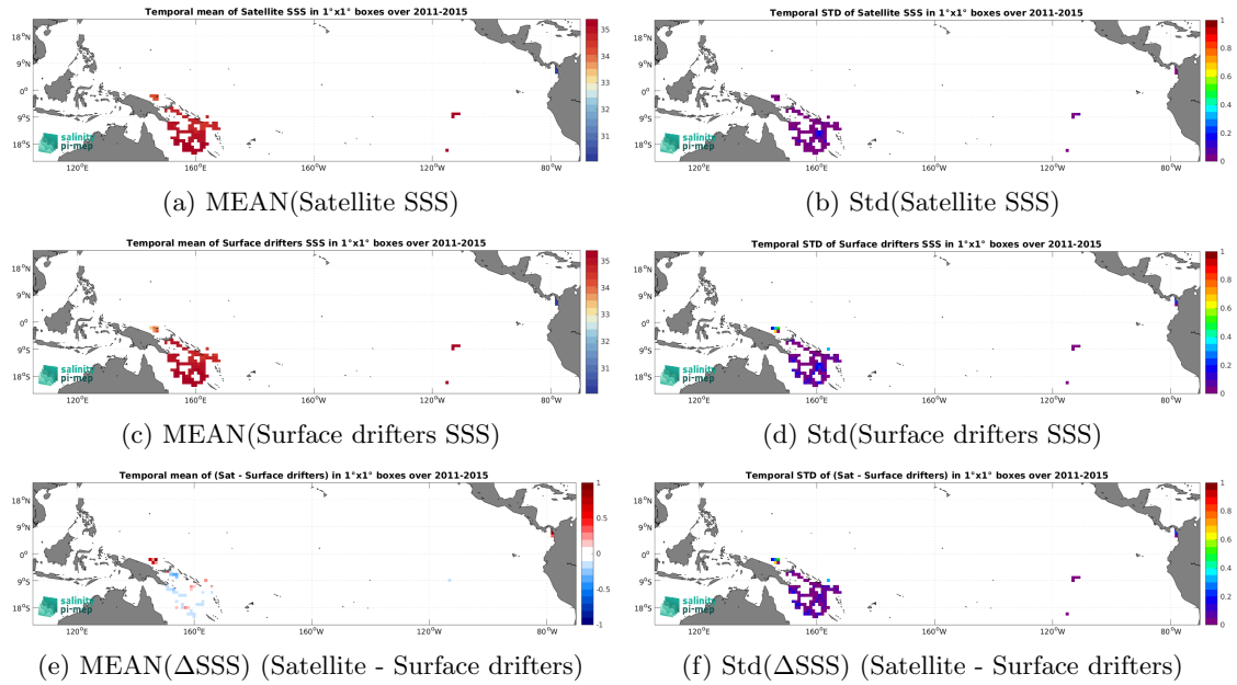
Figure 6: Temporal mean (left) and Std (right) of SSS from Aquarius SSS L4 OI v5 - Monthly (IPRC) (top), Surface drifters (middle), and of \Delta SSS (Satellite - Surface drifters). Only match-up pairs are used to generate these maps.
