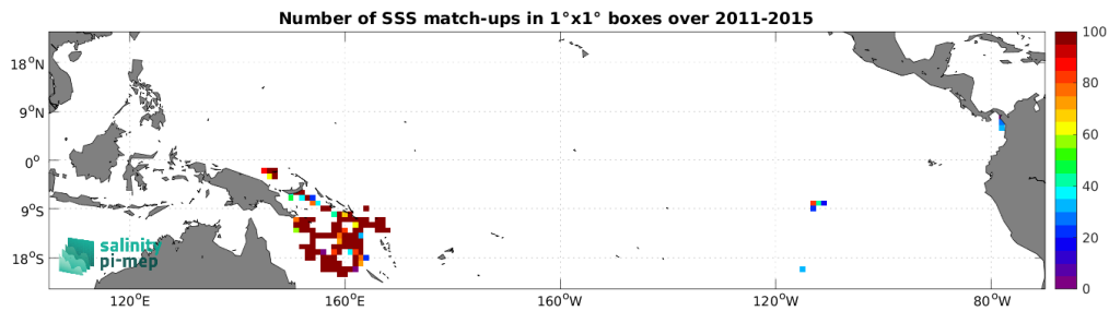
Figure 4: Number of SSS match-ups between Surface drifters SSS and the Aquarius SSS L4 OI v5 - Monthly (IPRC) SSS product for the Tropical Pacific Ocean Pi-MEP region over 1^\circ \times 1^\circ boxes and for the full satellite product period.
