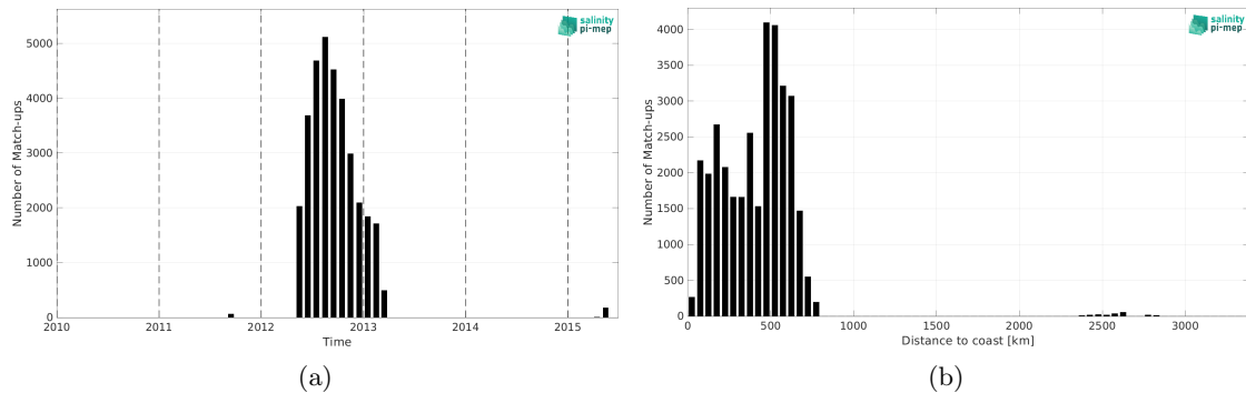
Figure 2: Number of match-ups between Surface drifters and Aquarius SSS L4 OI v5 - Monthly (IPRC) SSS as a function of time (a) and as function of the distance to coast (b) over the Tropical Pacific Ocean Pi-MEP region and for the full satellite product period.
