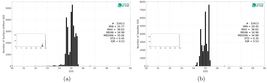
Figure 3: Histograms of SSS from Surface drifters (a) and Aquarius SSS L4 OI v5 - Monthly (IPRC) (b) considering all match-up pairs per bins of 0.1 over the Tropical Pacific Ocean Pi-MEP region and for the full satellite product period.
