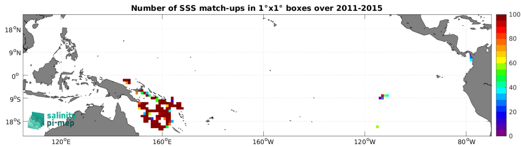
Figure 3: Number of SSS match-ups between Surface drifters SSS and the Aquarius SSS L4 OI v5 - Monthly (IPRC) SSS product for the Tropical Pacific Ocean Pi-MEP region over 1^\circ \times 1^\circ boxes and for the full satellite product period.
