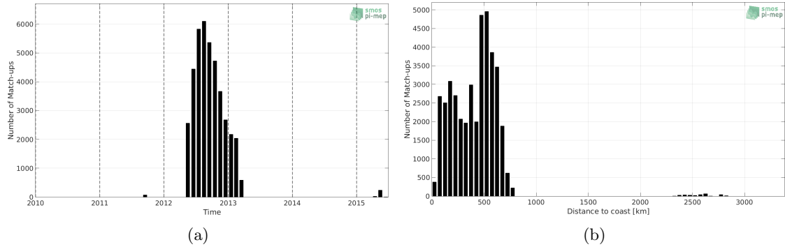
Figure 1: Number of match-ups between Surface drifters and Aquarius-L4-IPRC-V5-MONTHLY SSS as a function of time (a) and as function of the distance to coast (b) over the Tropical Pacific Ocean Pi-MEP region and for the full satellite product period.
