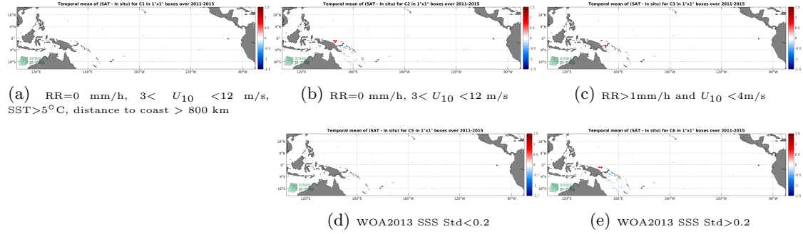
Figure 11: Temporal mean gridded over spatial boxes of size 1^\circ \times 1^\circ of \Delta SSS (Aquarius-L4-IPRC-V5-MONTHLY - Surface drifters) for 5 different subdatasets corresponding to: RR=0 mm/h, 3 < U_{10} < 12 m/s, SST >5^\circ\text{C} , distance to coast > 800 km (a), RR=0 mm/h, 3 < U_{10} < 12 m/s (b), RR >1 mm/h and U_{10} < 4 m/s (c), WOA2013 SSS Std <0.2 (d), WOA2013 SSS Std >0.2 (e).
