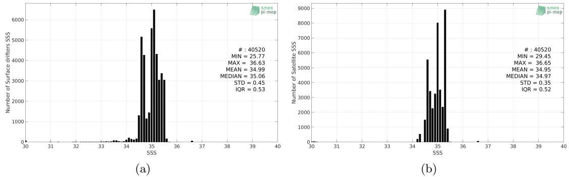
Figure 2: Histograms of SSS from Surface drifters (a) and Aquarius-L4-IPRC-V5-MONTHLY (b) considering all match-up pairs per bins of 0.1 over the Tropical Pacific Ocean Pi-MEP region and for the full satellite product period.
