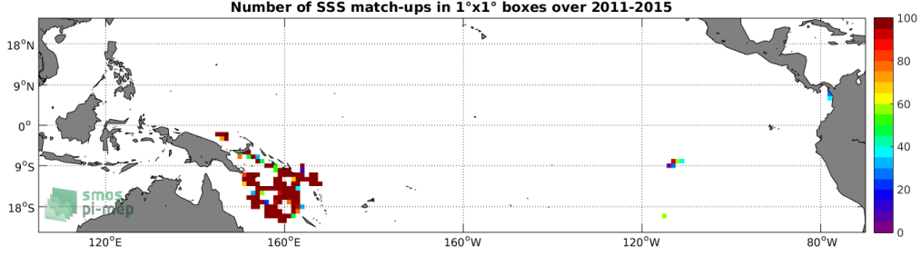
Figure 3: Number of SSS match-ups between Surface drifters SSS and the Aquarius-L4-IPRC-V5-MONTHLY SSS product for the Tropical Pacific Ocean Pi-MEP region over 1^\circ \times 1^\circ boxes and for the full satellite product period.
