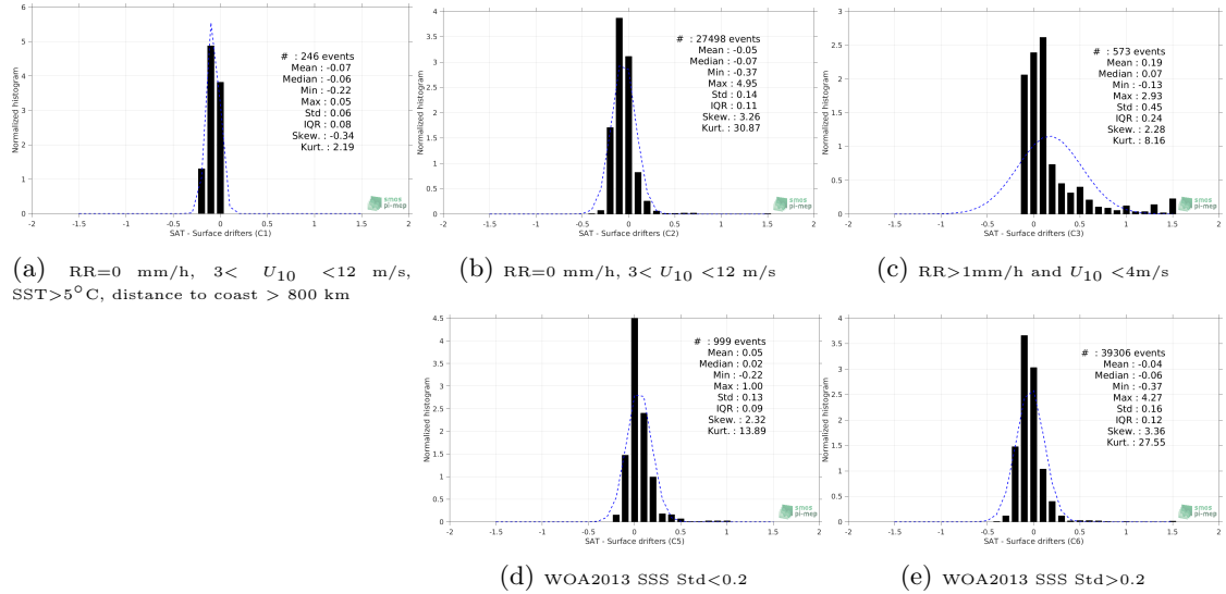
Figure 12: Normalized histogram of \Delta SSS (Aquarius-L4-IPRC-V5-MONTHLY - Surface drifters) for 5 different subdatasets corresponding to: RR=0 mm/h, 3 < U_{10} < 12 m/s, SST >5^\circ\text{C} , distance to coast > 800 km (a), RR=0 mm/h, 3 < U_{10} < 12 m/s (b), RR >1 mm/h and U_{10} < 4 m/s (c), WOA2013 SSS Std <0.2 (d), WOA2013 SSS Std >0.2 (e).
