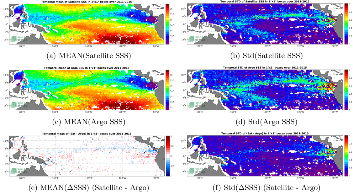
Figure 6: Temporal mean (left) and Std (right) of SSS from Aquarius-L4-IPRC-V5-MONTHLY (top), Argo (middle), and of \Delta SSS (Satellite - Argo). Only match-up pairs are used to generate these maps.
