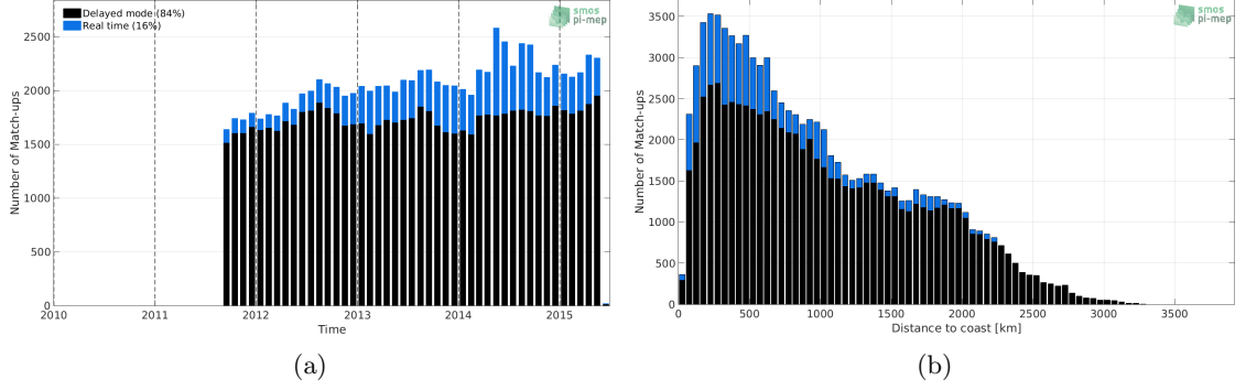
Figure 1: Number of match-ups between Argo and Aquarius-L4-IPRC-V5-MONTHLY SSS as a function of time (a) and as function of the distance to coast (b) over the Tropical Pacific Ocean Pi-MEP region and for the full satellite product period.
