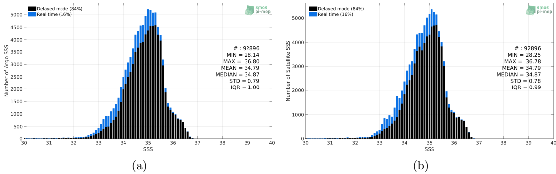
Figure 2: Histograms of SSS from Argo (a) and Aquarius-L4-IPRC-V5-MONTHLY (b) considering all match-up pairs per bins of 0.1 over the Tropical Pacific Ocean Pi-MEP region and for the full satellite product period.
