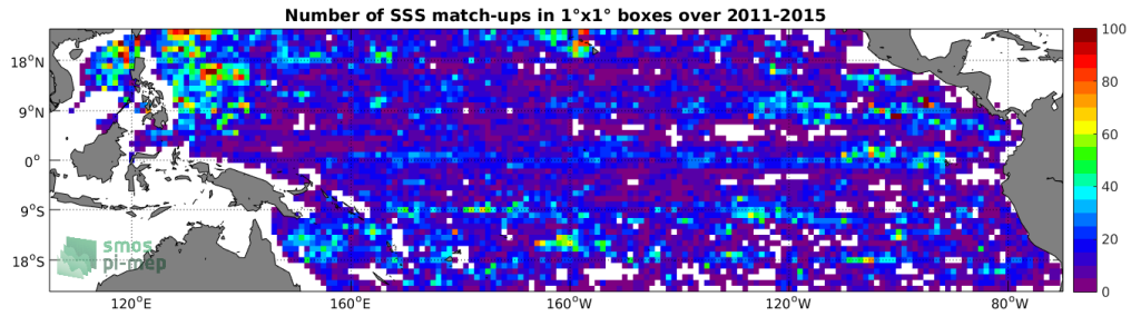
Figure 4: Number of SSS match-ups between Argo SSS and the Aquarius-L4-IPRC-V5-MONTHLY SSS product for the Tropical Pacific Ocean Pi-MEP region over 1^\circ \times 1^\circ boxes and for the full satellite product period.
