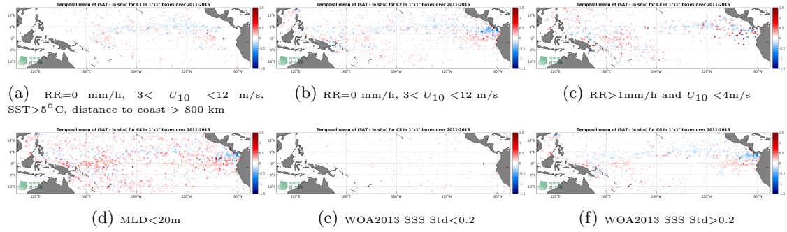
Figure 12: Temporal mean gridded over spatial boxes of size 1^\circ \times 1^\circ of \Delta SSS (Aquarius-L4-IPRC-V5-MONTHLY - Argo) for 6 different subdatasets corresponding to: RR=0 mm/h, 3 < U_{10} < 12 m/s, SST > 5^\circ C , distance to coast > 800 km (a), RR=0 mm/h, 3 < U_{10} < 12 m/s (b), RR > 1 mm/h and U_{10} < 4 m/s (c), MLD < 20 m (d), WOA2013 SSS Std < 0.2 (e), WOA2013 SSS Std > 0.2 (f).
