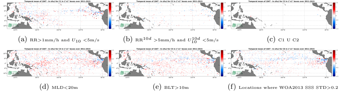
Figure 12: Temporal mean gridded over spatial boxes of size 1^\circ \times 1^\circ of \Delta\text{SSS} (Aquarius-L4-IPRC-V5-MONTHLY - Argo) for 6 different subdatasets corresponding to: \text{RR}>1\text{mm/h} and U_{10}<5\text{m/s} (a), \text{RR}^{10d}>5\text{mm/h} and U_{10d}<5\text{m/s} (b), C1 U C2 (c), \text{MLD}<20\text{m} (d), \text{BLT}>10\text{m} (e), Locations where WOA2013 SSS STD >0.2 (f).
