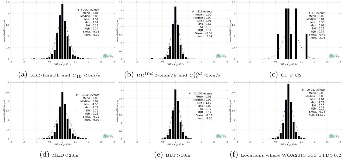
Figure 13: Normalized histogram of \Delta\text{SSS} (Aquarius-L4-IPRC-V5-MONTHLY - Argo) for 6 different subdatasets corresponding to: \text{RR}>1\text{mm/h} and U_{10}<5\text{m/s} (a), \text{RR}^{10d}>5\text{mm/h} and U_{10d}<5\text{m/s} (b), C1 U C2 (c), \text{MLD}<20\text{m} (d), \text{BLT}>10\text{m} (e), Locations where WOA2013 SSS STD >0.2 (f).
