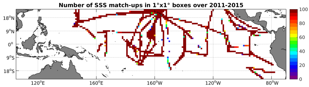
Figure 4: Number of SSS match-ups between TSG-SAMOS SSS and the Aquarius-L4-IPRC-V4-WEEKLY SSS product for the Tropical Pacific Ocean Pi-MEP region over 1^\circ \times 1^\circ boxes and for the full satellite product period.
