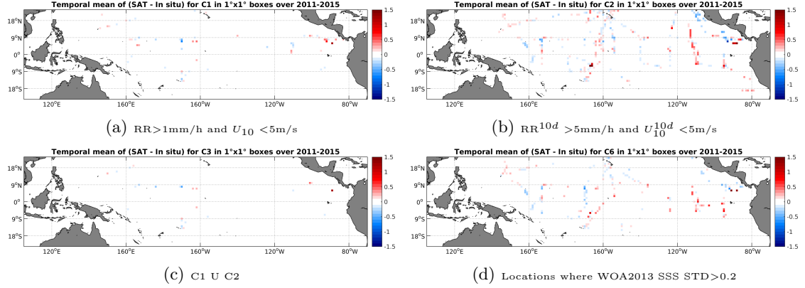
Figure 12: Temporal mean gridded over spatial boxes of size 1^\circ \times 1^\circ of \Delta SSS (Aquarius-L4-IPRC-V4-WEEKLY - TSG-SAMOS) for 4 different subdatasets corresponding to: RR > 1mm/h and U_{10} < 5 m/s (a), RR^{10d} > 5 mm/h and U_{10}^{10d} < 5 m/s (b), C1 U C2 (c), Locations where WOA2013 SSS STD > 0.2 (d).
