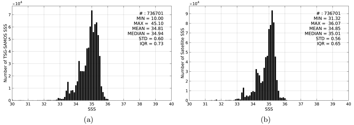
Figure 2: Histograms of SSS from TSG-SAMOS (a) and Aquarius-L4-IPRC-V4-WEEKLY (b) considering all match-up pairs per bins of 0.1 over the Tropical Pacific Ocean Pi-MEP region and for the full satellite product period.
