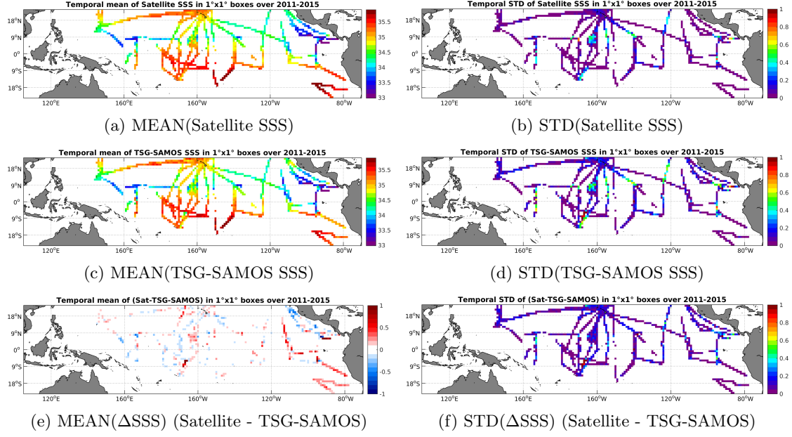
Figure 6: Temporal mean (left) and STD (right) of SSS from Aquarius-L4-IPRC-V4-WEEKLY (top), TSG-SAMOS (middle), and of \Delta SSS (Satellite - TSG-SAMOS). Only match-up pairs are used to generate these maps.
