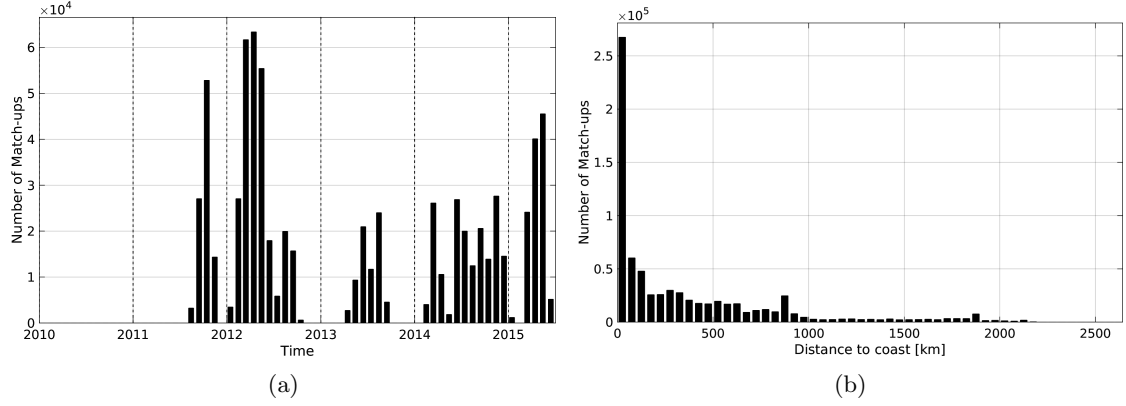
Figure 1: Number of match-ups between TSG-SAMOS and Aquarius-L4-IPRC-V4-WEEKLY SSS as a function of time (a) and as function of the distance to coast (b) over the Tropical Pacific Ocean Pi-MEP region and for the full satellite product period.
