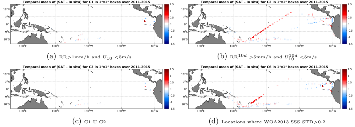
Figure 12: Temporal mean gridded over spatial boxes of size 1^\circ \times 1^\circ of \Delta SSS (Aquarius-L4-IPRC-V4-WEEKLY - TSG-GOSUD-Research-vessel) for 4 different subdatasets corresponding to: RR > 1 mm/h and U_{10} < 5 m/s (a), RR^{10d} > 5 mm/h and U_{10}^{10d} < 5 m/s (b), C1 U C2 (c), Locations where WOA2013 SSS STD > 0.2 (d).
