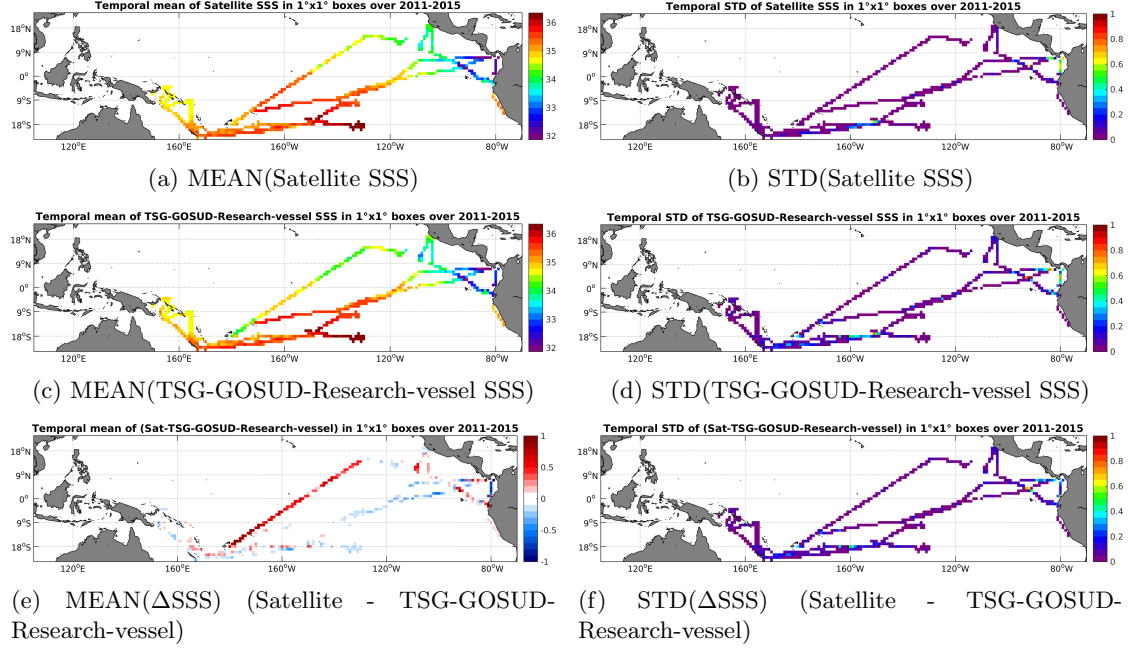
Figure 6: Temporal mean (left) and STD (right) of SSS from Aquarius-L4-IPRC-V4-WEEKLY (top), TSG-GOSUD-Research-vessel (middle), and of \Delta SSS (Satellite - TSG-GOSUD-Research-vessel). Only match-up pairs are used to generate these maps.
