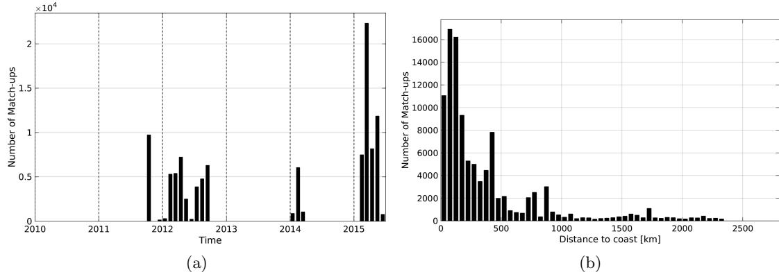
Figure 1: Number of match-ups between TSG-GOSUD-Research-vessel and Aquarius-L4-IPRC-V4-WEEKLY SSS as a function of time (a) and as function of the distance to coast (b) over the Tropical Pacific Ocean Pi-MEP region and for the full satellite product period.
