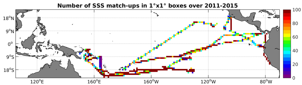
Figure 4: Number of SSS match-ups between TSG-GOSUD-Research-vessel SSS and the Aquarius-L4-IPRC-V4-WEEKLY SSS product for the Tropical Pacific Ocean Pi-MEP region over 1^\circ \times 1^\circ boxes and for the full satellite product period.
