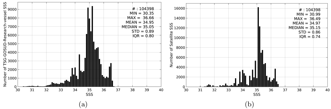
Figure 2: Histograms of SSS from TSG-GOSUD-Research-vessel (a) and Aquarius-L4-IPRC-V4-WEEKLY (b) considering all match-up pairs per bins of 0.1 over the Tropical Pacific Ocean Pi-MEP region and for the full satellite product period.
