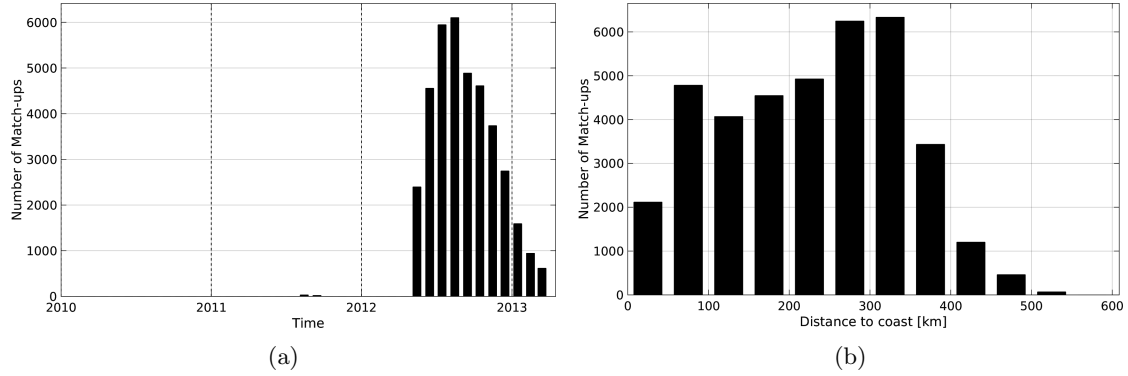
Figure 1: Number of match-ups between Surface drifters and Aquarius-L4-IPRC-V4-WEEKLY SSS as a function of time (a) and as function of the distance to coast (b) over the Tropical Pacific Ocean Pi-MEP region and for the full satellite product period.
