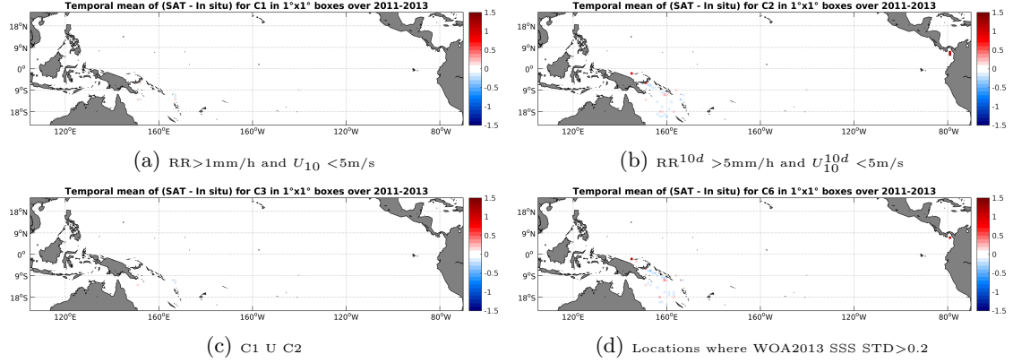
Figure 11: Temporal mean gridded over spatial boxes of size 1^\circ \times 1^\circ of \Delta SSS (Aquarius-L4-IPRC-V4-WEEKLY - Surface drifters) for 4 different subdatasets corresponding to: RR > 1\text{mm/h} and U_{10} < 5\text{m/s} (a), RR^{10d} > 5\text{mm/h} and U_{10}^{10d} < 5\text{m/s} (b), C1 U C2 (c), Locations where WOA2013 SSS STD > 0.2 (d).
