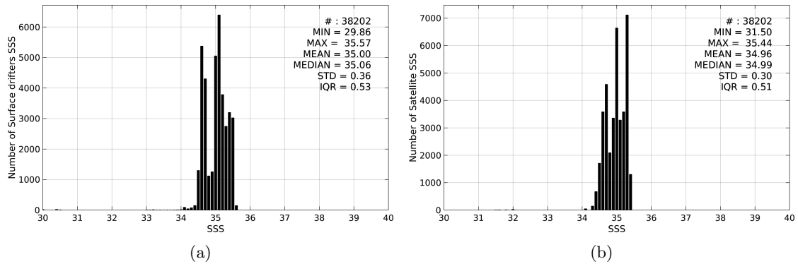
Figure 2: Histograms of SSS from Surface drifters (a) and Aquarius-L4-IPRC-V4-WEEKLY (b) considering all match-up pairs per bins of 0.1 over the Tropical Pacific Ocean Pi-MEP region and for the full satellite product period.
