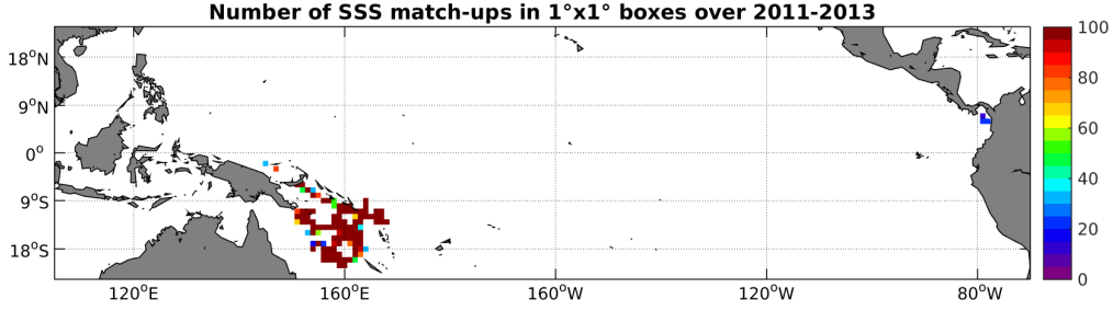
Figure 3: Number of SSS match-ups between Surface drifters SSS and the Aquarius-L4-IPRC-V4-WEEKLY SSS product for the Tropical Pacific Ocean Pi-MEP region over 1^\circ \times 1^\circ boxes and for the full satellite product period.
