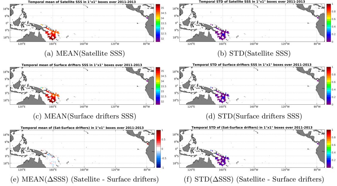
Figure 5: Temporal mean (left) and STD (right) of SSS from Aquarius-L4-IPRC-V4-WEEKLY (top), Surface drifters (middle), and of \Delta SSS (Satellite - Surface drifters). Only match-up pairs are used to generate these maps.
