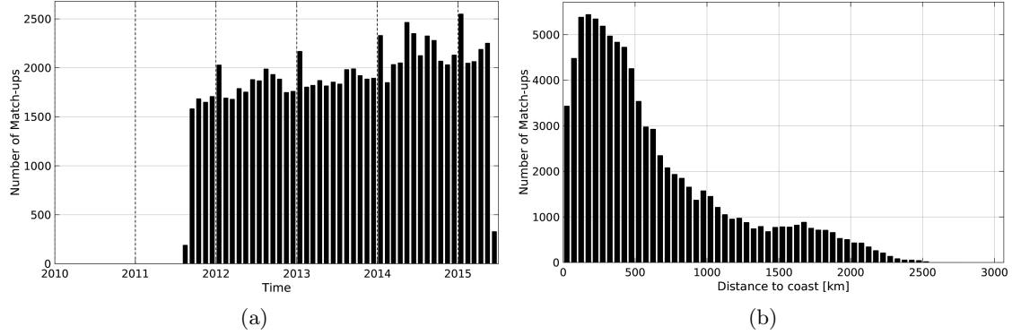
Figure 1: Number of match-ups between Argo and Aquarius-L4-IPRC-V4-WEEKLY SSS as a function of time (a) and as function of the distance to coast (b) over the Tropical Pacific Ocean Pi-MEP region and for the full satellite product period.
