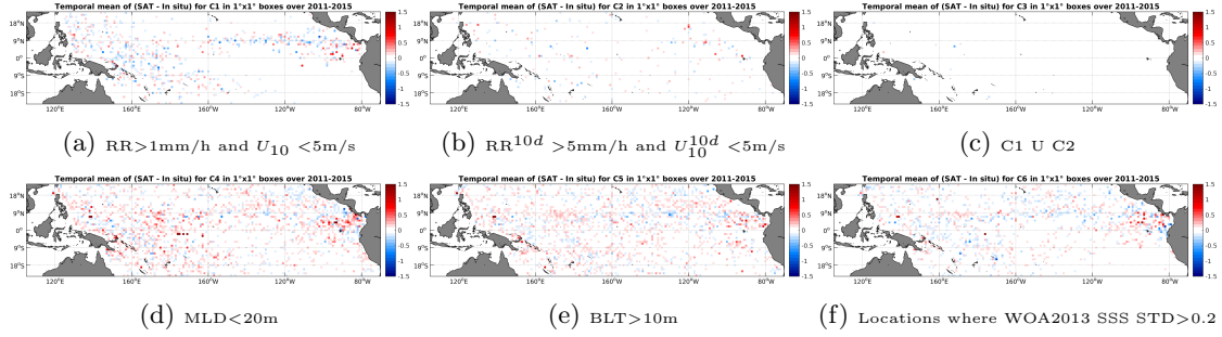
Figure 12: Temporal mean gridded over spatial boxes of size 1^\circ \times 1^\circ of \Delta SSS (Aquarius-L4-IPRC-V4-WEEKLY - Argo) for 6 different subdatasets corresponding to: RR > 1\text{mm/h} and U_{10} < 5\text{m/s} (a), RR^{10d} > 5\text{mm/h} and U_{10}^{10d} < 5\text{m/s} (b), C1 U C2 (c), MLD < 20\text{m} (d), BLT > 10\text{m} (e), Locations where WOA2013 SSS STD > 0.2 (f).
