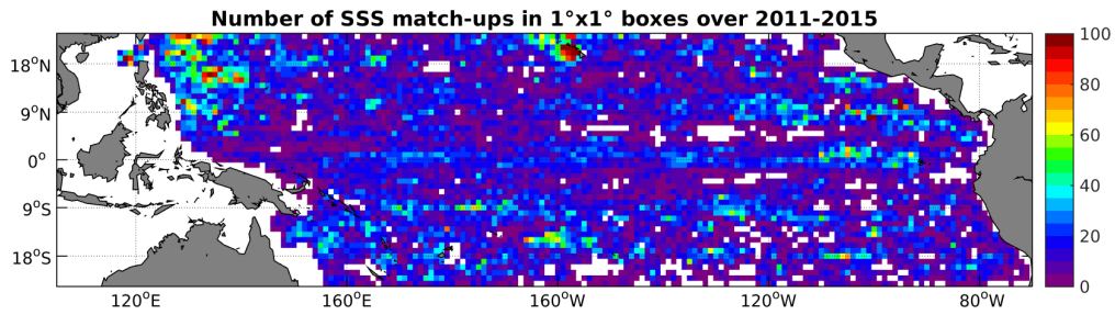
Figure 4: Number of SSS match-ups between Argo SSS and the Aquarius-L4-IPRC-V4-WEEKLY SSS product for the Tropical Pacific Ocean Pi-MEP region over 1°x1° boxes and for the full satellite product period.
