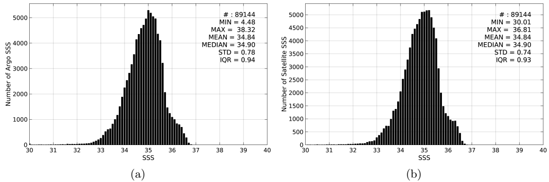
Figure 2: Histograms of SSS from Argo (a) and Aquarius-L4-IPRC-V4-WEEKLY (b) considering all match-up pairs per bins of 0.1 over the Tropical Pacific Ocean Pi-MEP region and for the full satellite product period.
