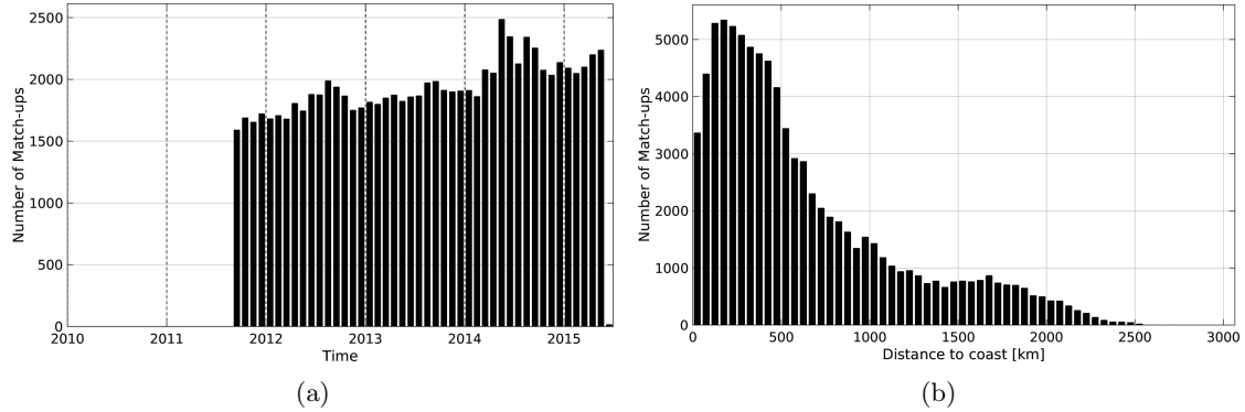
Figure 1: Number of match-ups between Argo and Aquarius-L4-IPRC-V4-MONTHLY SSS as a function of time (a) and as function of the distance to coast (b) over the Tropical Pacific Ocean Pi-MEP region and for the full satellite product period.
