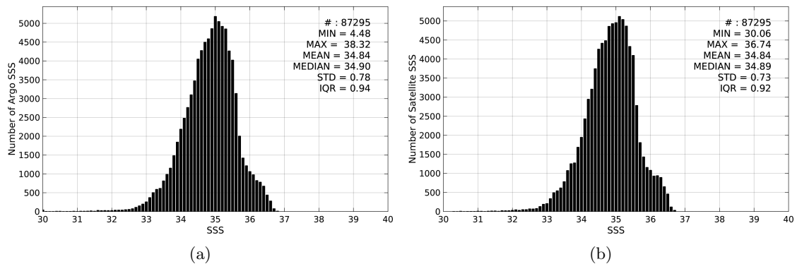
Figure 2: Histograms of SSS from Argo (a) and Aquarius-L4-IPRC-V4-MONTHLY (b) considering all match-up pairs per bins of 0.1 over the Tropical Pacific Ocean Pi-MEP region and for the full satellite product period.
