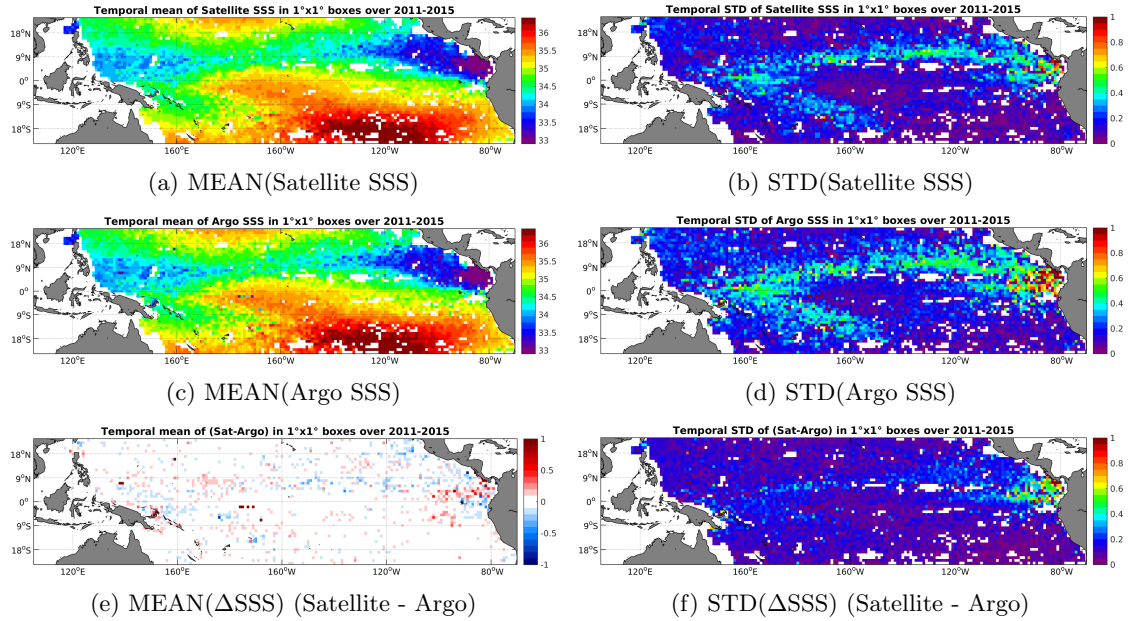
Figure 6: Temporal mean (left) and STD (right) of SSS from Aquarius-L4-IPRC-V4-MONTHLY (top), Argo (middle), and of \Delta SSS (Satellite - Argo). Only match-up pairs are used to generate these maps.
