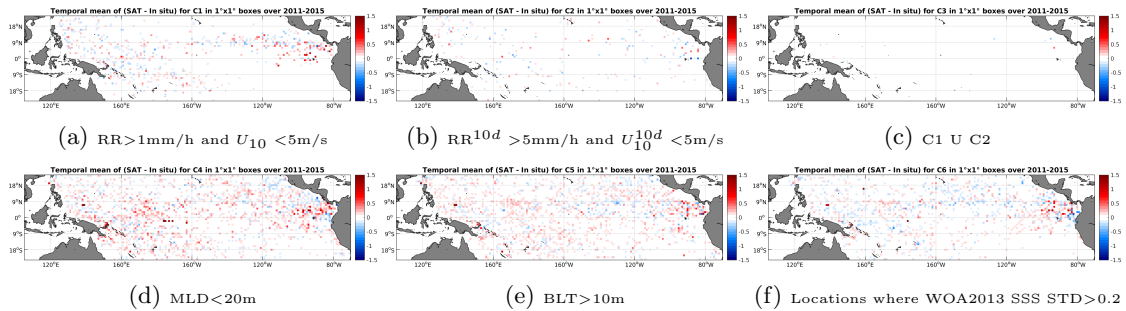
Figure 12: Temporal mean gridded over spatial boxes of size 1°x1° of \Delta SSS (Aquarius-L4-IPRC-V4-MONTHLY - Argo) for 6 different subdatasets corresponding to:RR>1mm/h and U_{10} < 5 m/s (a), RR^{10d} > 5 mm/h and U_{10}^{10d} < 5 m/s (b), C1 U C2 (c),MLD<20m (d),BLT>10m (e),Locations where WOA2013 SSS STD>0.2 (f).
