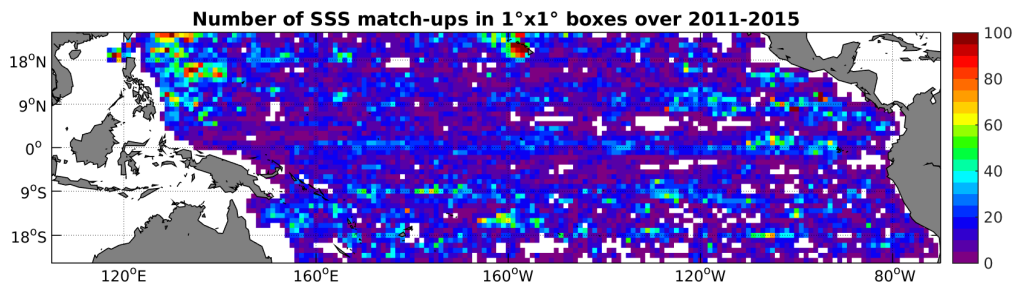
Figure 4: Number of SSS match-ups between Argo SSS and the Aquarius-L4-IPRC-V4-MONTHLY SSS product for the Tropical Pacific Ocean Pi-MEP region over 1^\circ \times 1^\circ boxes and for the full satellite product period.
