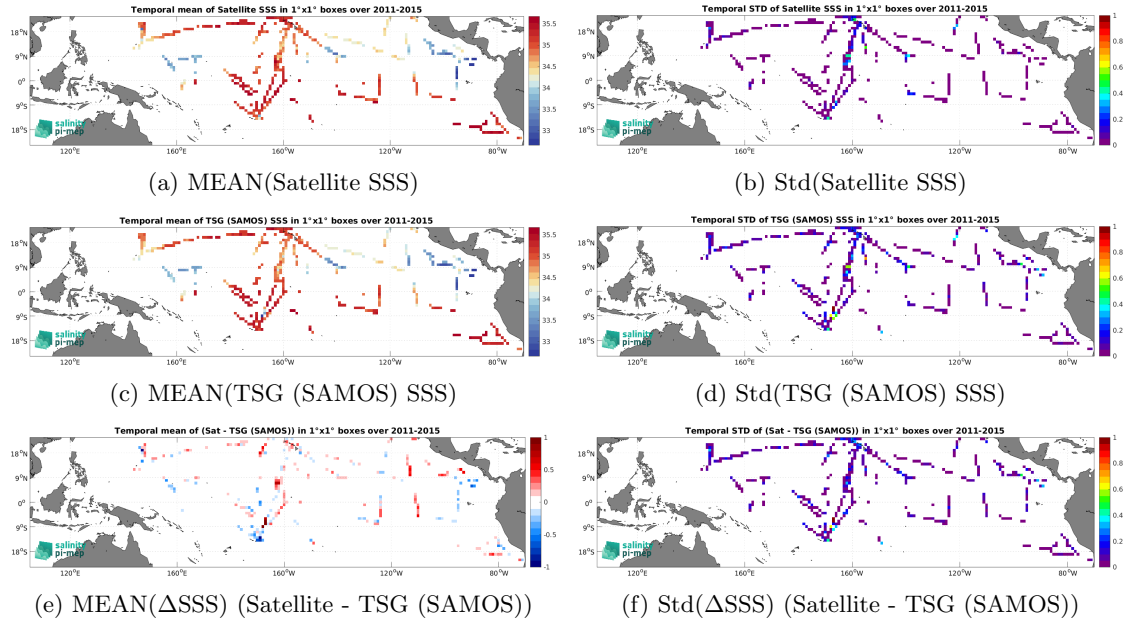
Figure 7: Temporal mean (left) and Std (right) of SSS from Aquarius SSS L3 OR v5 - 7-Day running (NASA-GSFC) (top), TSG (SAMOS) (middle), and of \Delta SSS (Satellite - TSG (SAMOS)). Only match-up pairs are used to generate these maps.
