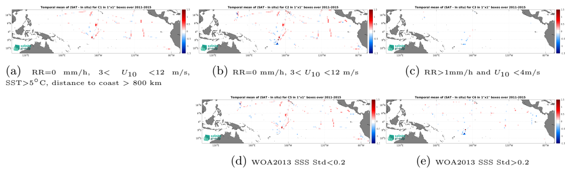
Figure 14: Temporal mean gridded over spatial boxes of size 1^\circ \times 1^\circ of \Delta SSS (Aquarius SSS L3 OR v5 - 7-Day running (NASA-GSFC) - TSG (SAMOS)) for 5 different subdatasets corresponding to: RR=0 mm/h, 3 < U_{10} < 12 m/s, SST > 5^\circ\text{C} , distance to coast > 800 km (a), RR=0 mm/h, 3 < U_{10} < 12 m/s (b), RR > 1 mm/h and U_{10} < 4 m/s (c), WOA2013 SSS Std < 0.2 (d), WOA2013 SSS Std > 0.2 (e).
