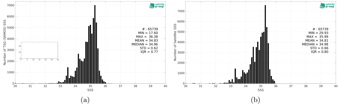
Figure 2: Histograms of SSS from TSG (SAMOS) (a) and Aquarius SSS L3 OR v5 - 7-Day running (NASA-GSFC) (b) considering all match-up pairs per bins of 0.1 over the Tropical Pacific Ocean Pi-MEP region and for the full satellite product period.
