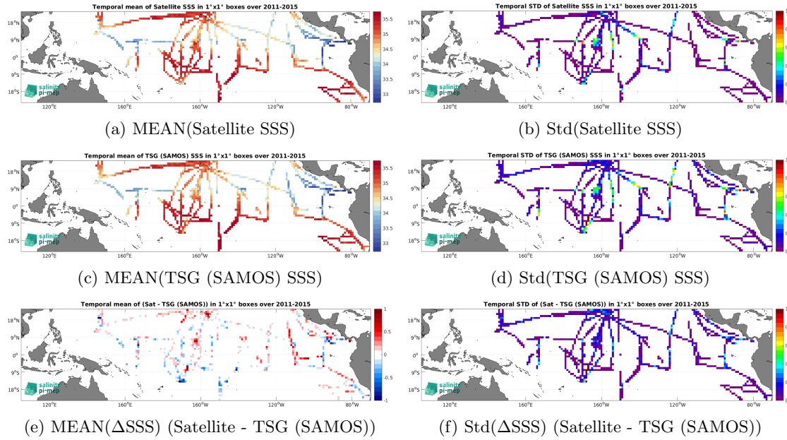
Figure 6: Temporal mean (left) and Std (right) of SSS from Aquarius SSS L3 OR v5 - 7-Day running (NASA-GSFC) (top), TSG (SAMOS) (middle), and of \Delta SSS (Satellite - TSG (SAMOS)). Only match-up pairs are used to generate these maps.
