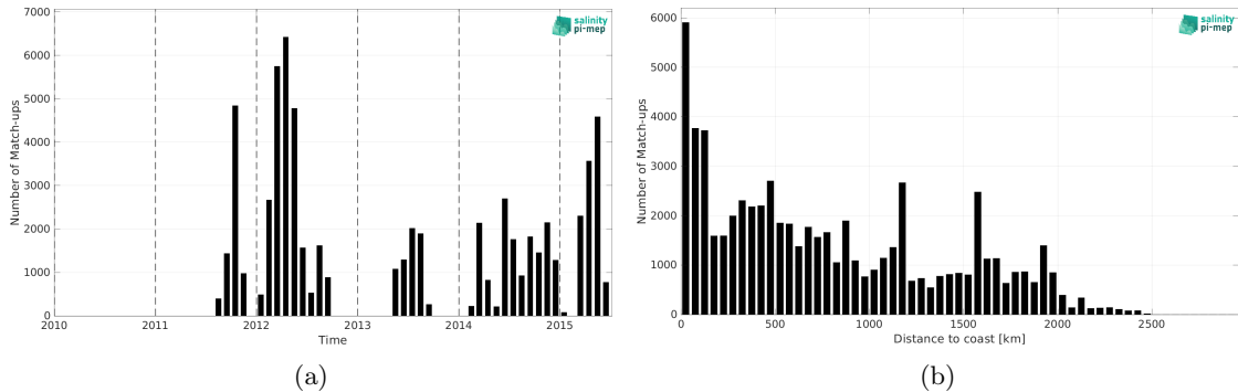
Figure 1: Number of match-ups between TSG (SAMOS) and Aquarius SSS L3 OR v5 - 7-Day running (NASA-GSFC) SSS as a function of time (a) and as function of the distance to coast (b) over the Tropical Pacific Ocean Pi-MEP region and for the full satellite product period.
