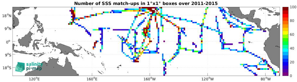
Figure 4: Number of SSS match-ups between TSG (SAMOS) SSS and the Aquarius SSS L3 OR v5 - 7-Day running (NASA-GSFC) SSS product for the Tropical Pacific Ocean Pi-MEP region over 1^\circ \times 1^\circ boxes and for the full satellite product period.
