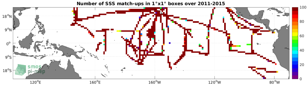
Figure 4: Number of SSS match-ups between TSG (SAMOS) SSS and the Aquarius SSS L3 OR v5 - 7-Day running (NASA-GSFC) SSS product for the Tropical Pacific Ocean Pi-MEP region over 1^\circ \times 1^\circ boxes and for the full satellite product period.
