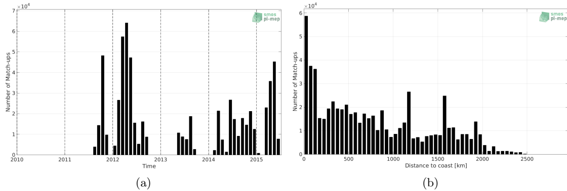
Figure 1: Number of match-ups between TSG (SAMOS) and Aquarius SSS L3 OR v5 - 7-Day running (NASA-GSFC) SSS as a function of time (a) and as function of the distance to coast (b) over the Tropical Pacific Ocean Pi-MEP region and for the full satellite product period.
