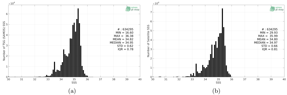
Figure 2: Histograms of SSS from TSG (SAMOS) (a) and Aquarius SSS L3 OR v5 - 7-Day running (NASA-GSFC) (b) considering all match-up pairs per bins of 0.1 over the Tropical Pacific Ocean Pi-MEP region and for the full satellite product period.
