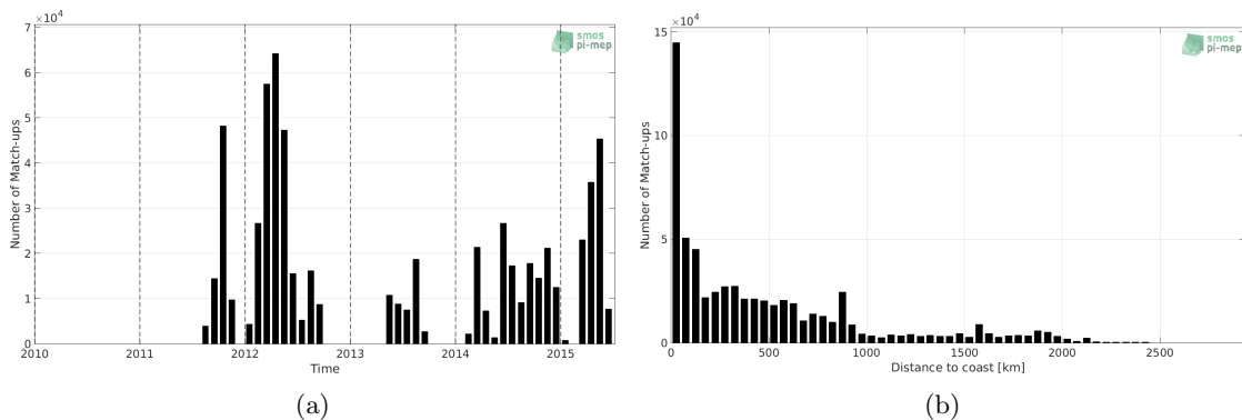
Figure 1: Number of match-ups between TSG-SAMOS and Aquarius-L3-OR-V5-7DAY-RUNNING-1DEG SSS as a function of time (a) and as function of the distance to coast (b) over the Tropical Pacific Ocean Pi-MEP region and for the full satellite product period.
