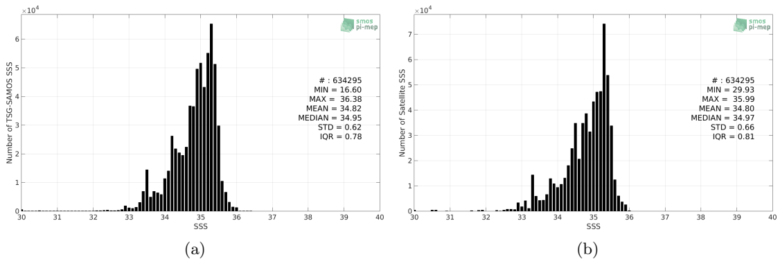
Figure 2: Histograms of SSS from TSG-SAMOS (a) and Aquarius-L3-OR-V5-7DAY-RUNNING-1DEG (b) considering all match-up pairs per bins of 0.1 over the Tropical Pacific Ocean Pi-MEP region and for the full satellite product period.
