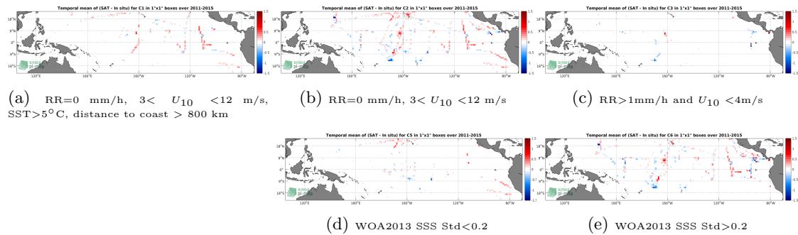
Figure 12: Temporal mean gridded over spatial boxes of size 1^\circ \times 1^\circ of \Delta SSS (Aquarius-L3-OR-V5-7DAY-RUNNING-1DEG - TSG-SAMOS) for 5 different subdatasets corresponding to: RR=0 mm/h, 3 < U_{10} < 12 m/s, SST > 5^\circ C , distance to coast > 800 km (a), RR=0 mm/h, 3 < U_{10} < 12 m/s (b), RR > 1 mm/h and U_{10} < 4 m/s (c), WOA2013 SSS Std < 0.2 (d), WOA2013 SSS Std > 0.2 (e).
