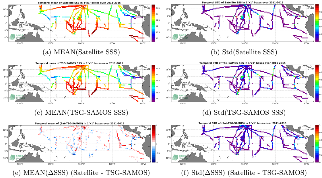
Figure 6: Temporal mean (left) and Std (right) of SSS from Aquarius-L3-OR-V5-7DAY-RUNNING-1DEG (top), TSG-SAMOS (middle), and of \Delta SSS (Satellite - TSG-SAMOS). Only match-up pairs are used to generate these maps.
