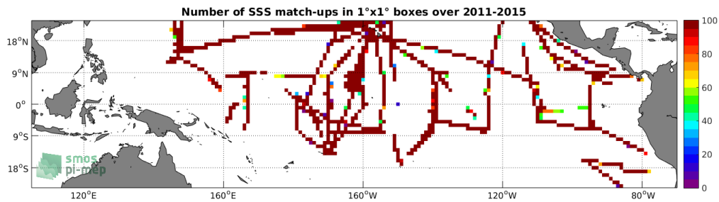
Figure 4: Number of SSS match-ups between TSG-SAMOS SSS and the Aquarius-L3-OR-V5-7DAY-RUNNING-1DEG SSS product for the Tropical Pacific Ocean Pi-MEP region over 1^\circ \times 1^\circ boxes and for the full satellite product period.
