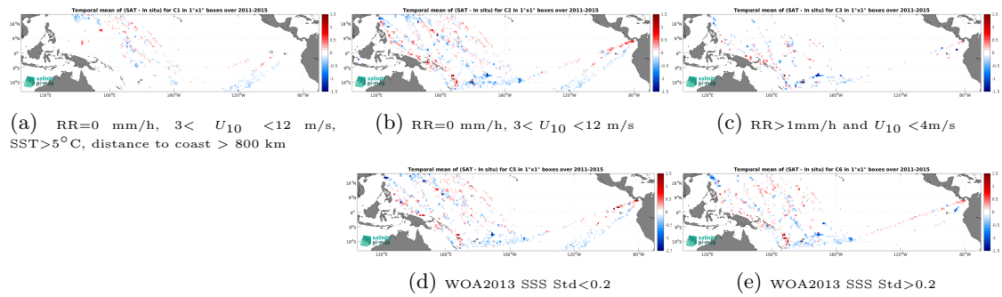
Figure 12: Temporal mean gridded over spatial boxes of size 1^\circ \times 1^\circ of \Delta\text{SSS} (Aquarius SSS L3 OR v5 - 7-Day running (NASA-GSFC) - TSG (LEGOS-DM)) for 5 different subdatasets corresponding to: RR=0 mm/h, 3 < U_{10} < 12 m/s, SST > 5^\circ\text{C} , distance to coast > 800 km (a), RR=0 mm/h, 3 < U_{10} < 12 m/s (b), RR > 1\text{mm/h} and U_{10} < 4\text{m/s} (c), WOA2013 SSS Std < 0.2 (d), WOA2013 SSS Std > 0.2 (e).
