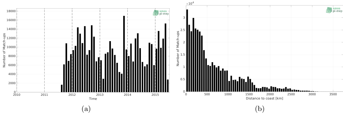
Figure 1: Number of match-ups between TSG (LEGOS-DM) and Aquarius SSS L3 OR v5 - 7-Day running (NASA-GSFC) SSS as a function of time (a) and as function of the distance to coast (b) over the Tropical Pacific Ocean Pi-MEP region and for the full satellite product period.
