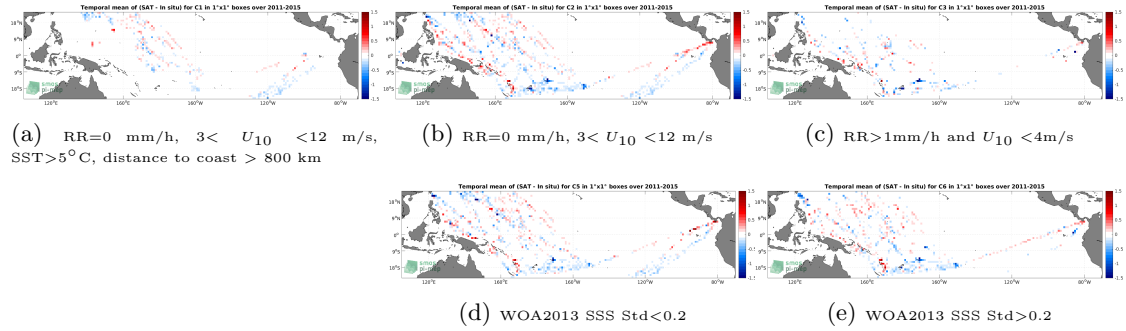
Figure 12: Temporal mean gridded over spatial boxes of size 1^{\circ}\times 1^{\circ} of \Delta\text{SSS} (Aquarius SSS L3 OR v5 - 7-Day running (NASA-GSFC) - TSG (LEGOS-DM)) for 5 different subdatasets corresponding to:RR=0 mm/h, 3 < U_{10} < 12 m/s, SST >5^{\circ}\text{C} , distance to coast > 800 km (a), RR=0 mm/h, 3 < U_{10} < 12 m/s (b), RR >1 mm/h and U_{10} < 4 m/s (c), WOA2013 SSS Std <0.2 (d), WOA2013 SSS Std >0.2 (e).
