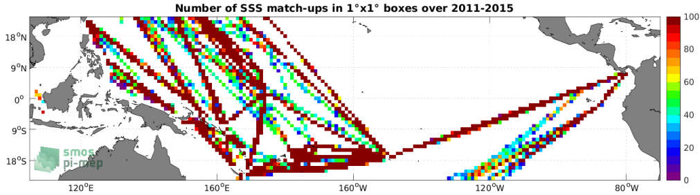
Figure 4: Number of SSS match-ups between TSG (LEGOS-DM) SSS and the Aquarius SSS L3 OR v5 - 7-Day running (NASA-GSFC) SSS product for the Tropical Pacific Ocean Pi-MEP region over 1^\circ \times 1^\circ boxes and for the full satellite product period.
