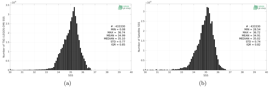
Figure 2: Histograms of SSS from TSG (LEGOS-DM) (a) and Aquarius SSS L3 OR v5 - 7-Day running (NASA-GSFC) (b) considering all match-up pairs per bins of 0.1 over the Tropical Pacific Ocean Pi-MEP region and for the full satellite product period.
