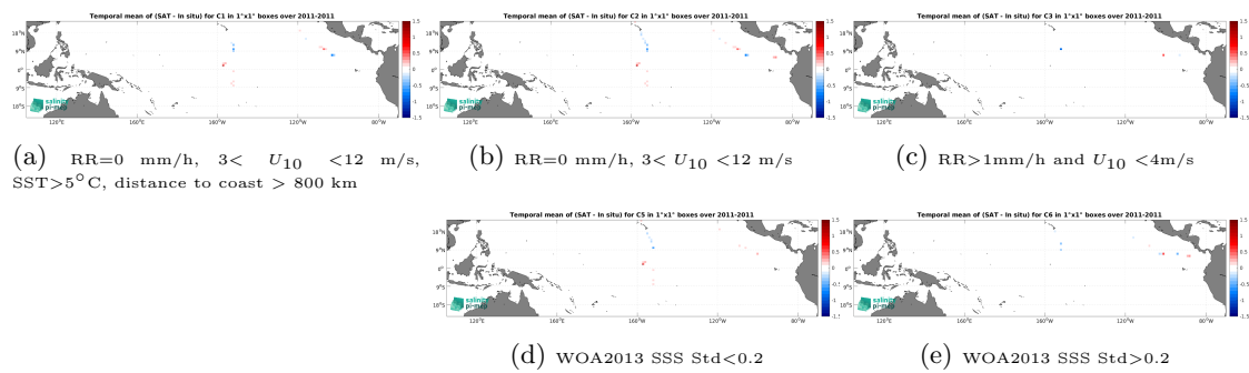
Figure 14: Temporal mean gridded over spatial boxes of size 1^\circ \times 1^\circ of \Delta SSS (Aquarius SSS L3 OR v5 - 7-Day running (NASA-GSFC) - TSG (GOSUD-Sailing-ship)) for 5 different subdatasets corresponding to: RR=0 mm/h, 3 < U_{10} < 12 m/s, SST > 5^\circ\text{C} , distance to coast > 800 km (a), RR=0 mm/h, 3 < U_{10} < 12 m/s (b), RR > 1 mm/h and U_{10} < 4 m/s (c), WOA2013 SSS Std < 0.2 (d), WOA2013 SSS Std > 0.2 (e).
