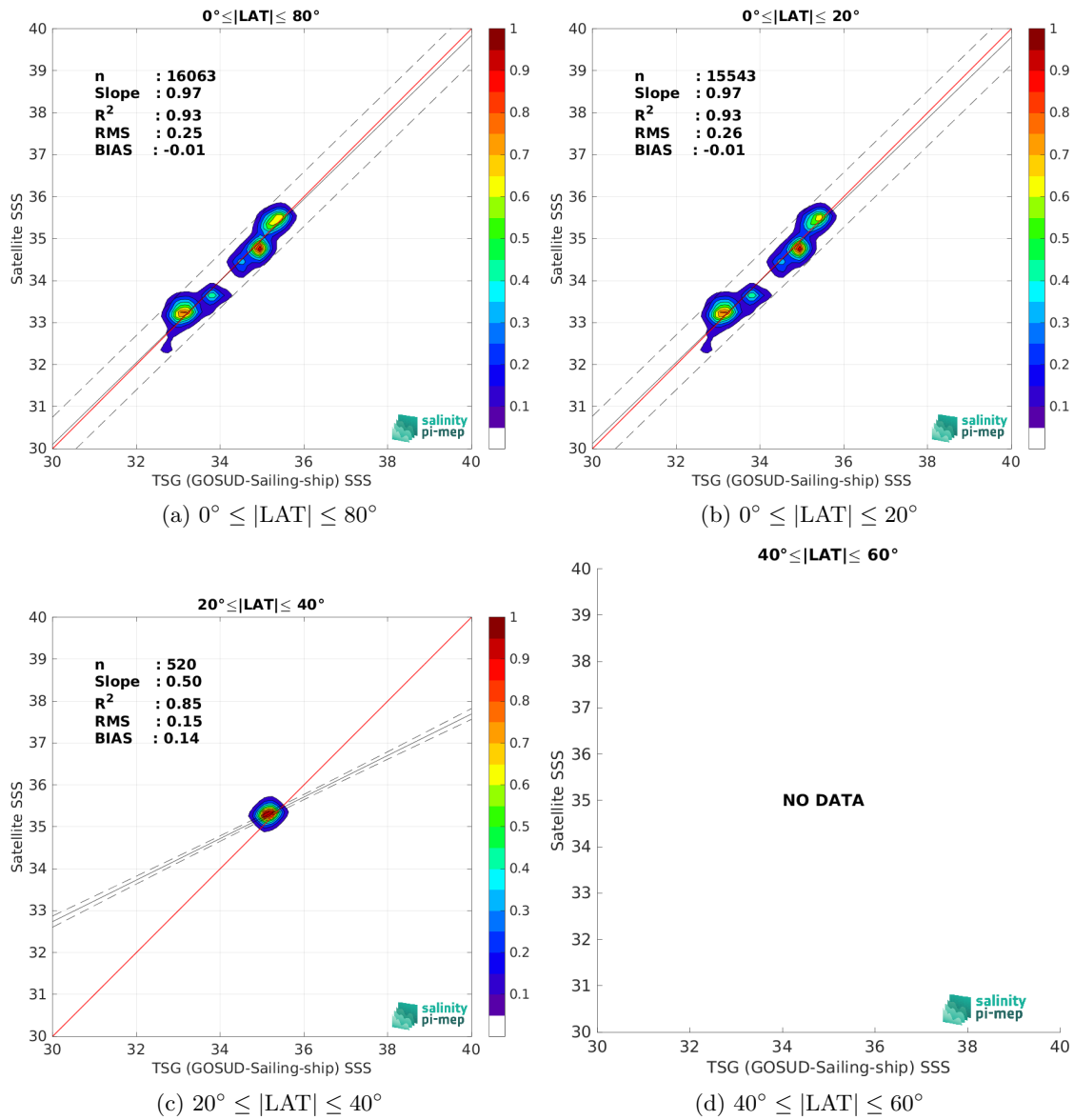
Figure 10: Contour maps of the concentration of Aquarius SSS L3 OR v5 - 7-Day running (NASA-GSFC) SSS (y-axis) versus TSG (GOSUD-Sailing-ship) SSS (x-axis) at match-up pairs for different latitude bands. For each plot, the red line shows x=y . The black thin and dashed lines indicate a linear fit through the data cloud and the \pm 95\% confidence levels, respectively. The number match-up pairs n , the slope and R^2 coefficient of the linear fit, the root mean square (RMS) and the mean bias between satellite and in situ data are indicated for each latitude band in each plots.
