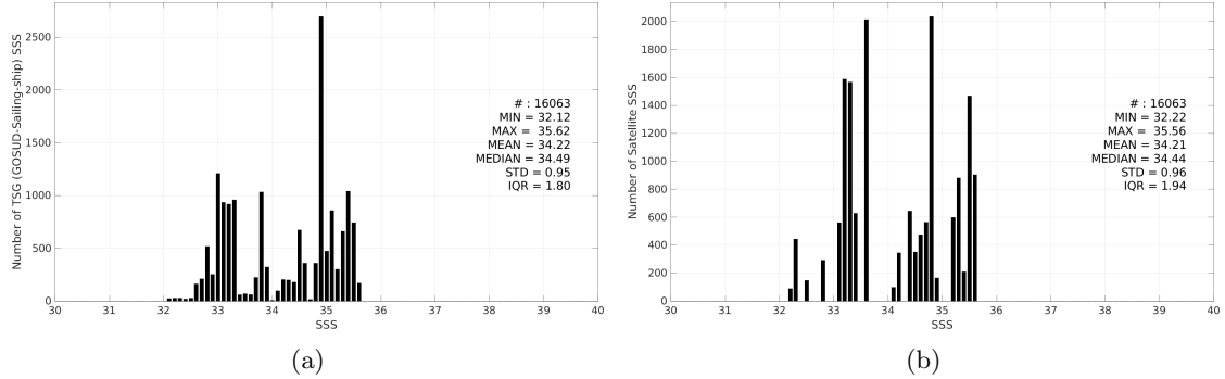
Figure 3: Histograms of SSS from TSG (GOSUD-Sailing-ship) (a) and Aquarius SSS L3 OR v5 - 7-Day running (NASA-GSFC) (b) considering all match-up pairs per bins of 0.1 over the Tropical Pacific Ocean Pi-MEP region and for the full satellite product period.
