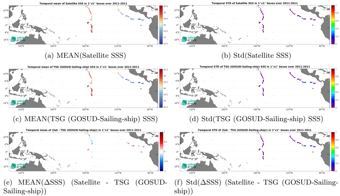
Figure 7: Temporal mean (left) and Std (right) of SSS from Aquarius SSS L3 OR v5 - 7-Day running (NASA-GSFC) (top), TSG (GOSUD-Sailing-ship) (middle), and of \Delta SSS (Satellite - TSG (GOSUD-Sailing-ship)). Only match-up pairs are used to generate these maps.
