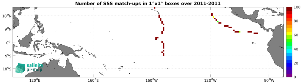
Figure 5: Number of SSS match-ups between TSG (GOSUD-Sailing-ship) SSS and the Aquarius SSS L3 OR v5 - 7-Day running (NASA-GSFC) SSS product for the Tropical Pacific Ocean Pi-MEP region over 1^\circ \times 1^\circ boxes and for the full satellite product period.
