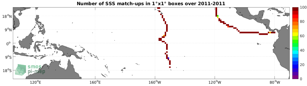
Figure 4: Number of SSS match-ups between TSG (GOSUD-Sailing-ship) SSS and the Aquarius SSS L3 OR v5 - 7-Day running (NASA-GSFC) SSS product for the Tropical Pacific Ocean Pi-MEP region over 1^\circ \times 1^\circ boxes and for the full satellite product period.
