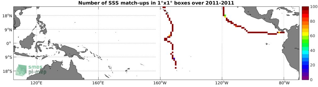
Figure 4: Number of SSS match-ups between TSG (GOSUD-Sailing-ship) SSS and the Aquarius SSS L3 OR v5 - 7-Day running (NASA-GSFC) SSS product for the Tropical Pacific Ocean Pi-MEP region over 1^\circ \times 1^\circ boxes and for the full satellite product period.
