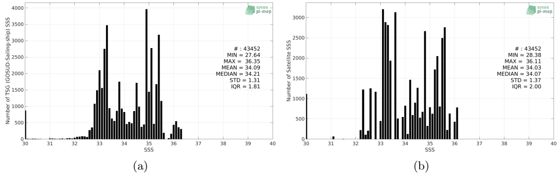
Figure 2: Histograms of SSS from TSG (GOSUD-Sailing-ship) (a) and Aquarius SSS L3 OR v5 - 7-Day running (NASA-GSFC) (b) considering all match-up pairs per bins of 0.1 over the Tropical Pacific Ocean Pi-MEP region and for the full satellite product period.
