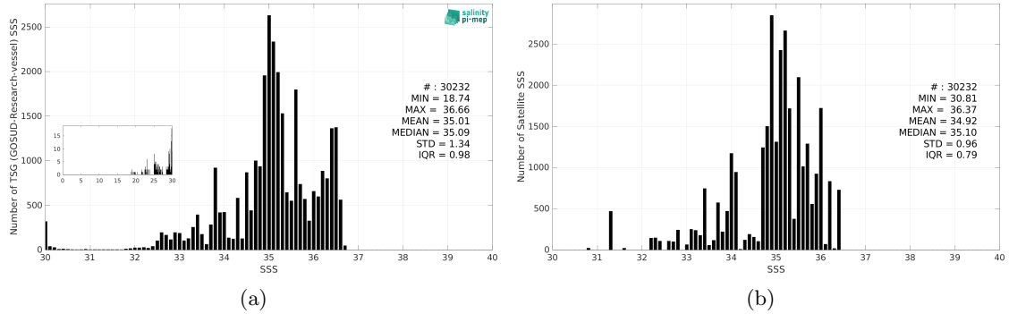
Figure 3: Histograms of SSS from TSG (GOSUD-Research-vessel) (a) and Aquarius SSS L3 OR v5 - 7-Day running (NASA-GSFC) (b) considering all match-up pairs per bins of 0.1 over the Tropical Pacific Ocean Pi-MEP region and for the full satellite product period.
