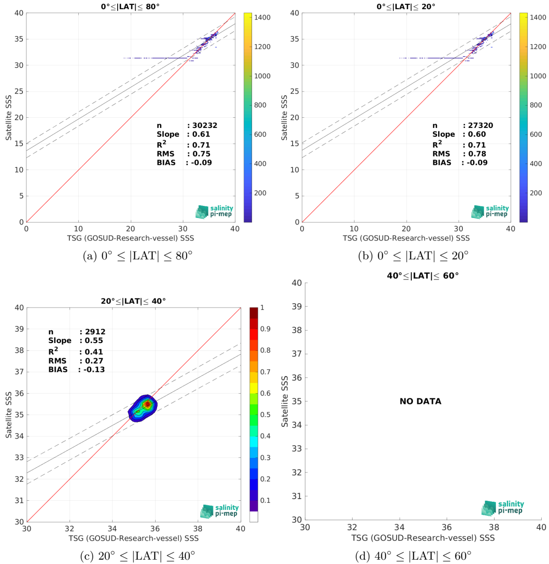
Figure 10: Contour maps of the concentration of Aquarius SSS L3 OR v5 - 7-Day running (NASA-GSFC) SSS (y-axis) versus TSG (GOSUD-Research-vessel) SSS (x-axis) at match-up pairs for different latitude bands. For each plot, the red line shows x=y . The black thin and dashed lines indicate a linear fit through the data cloud and the \pm 95\% confidence levels, respectively. The number match-up pairs n , the slope and R^2 coefficient of the linear fit, the root mean square (RMS) and the mean bias between satellite and in situ data are indicated for each latitude band in each plots.
