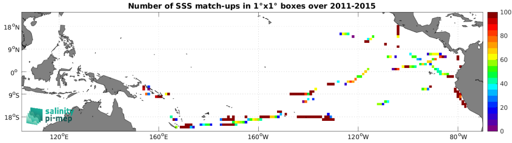
Figure 5: Number of SSS match-ups between TSG (GOSUD-Research-vessel) SSS and the Aquarius SSS L3 OR v5 - 7-Day running (NASA-GSFC) SSS product for the Tropical Pacific Ocean Pi-MEP region over 1^\circ \times 1^\circ boxes and for the full satellite product period.
