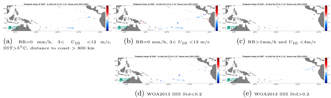
Figure 14: Temporal mean gridded over spatial boxes of size 1^\circ \times 1^\circ of \Delta SSS (Aquarius SSS L3 OR v5 - 7-Day running (NASA-GSFC) - TSG (GOSUD-Research-vessel)) for 5 different subdatasets corresponding to:RR=0 mm/h, 3 < U_{10} < 12 m/s, SST > 5^\circ\text{C} , distance to coast > 800 km (a), RR=0 mm/h, 3 < U_{10} < 12 m/s (b), RR > 1 mm/h and U_{10} < 4 m/s (c), WOA2013 SSS Std < 0.2 (d), WOA2013 SSS Std > 0.2 (e).
