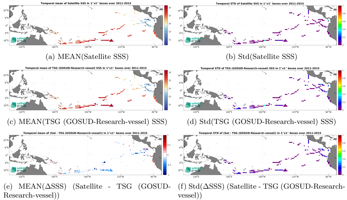
Figure 7: Temporal mean (left) and Std (right) of SSS from Aquarius SSS L3 OR v5 - 7-Day running (NASA-GSFC) (top), TSG (GOSUD-Research-vessel) (middle), and of \Delta SSS (Satellite - TSG (GOSUD-Research-vessel)). Only match-up pairs are used to generate these maps.
