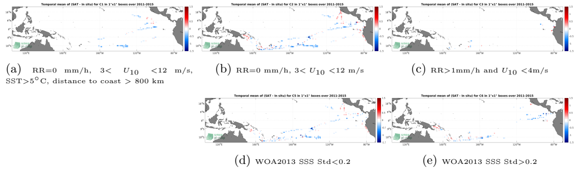
Figure 12: Temporal mean gridded over spatial boxes of size 1^{\circ}\times 1^{\circ} of \Delta SSS (Aquarius SSS L3 OR v5 - 7-Day running (NASA-GSFC) - TSG (GOSUD-Research-vessel)) for 5 different subdatasets corresponding to:RR=0 mm/h, 3 < U_{10} < 12 m/s, SST >5^{\circ}\text{C} , distance to coast > 800 km (a), RR=0 mm/h, 3 < U_{10} < 12 m/s (b), RR >1 mm/h and U_{10} < 4 m/s (c), WOA2013 SSS Std <0.2 (d), WOA2013 SSS Std >0.2 (e).
