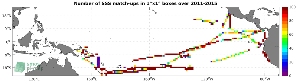
Figure 4: Number of SSS match-ups between TSG (GOSUD-Research-vessel) SSS and the Aquarius SSS L3 OR v5 - 7-Day running (NASA-GSFC) SSS product for the Tropical Pacific Ocean Pi-MEP region over 1^\circ \times 1^\circ boxes and for the full satellite product period.
