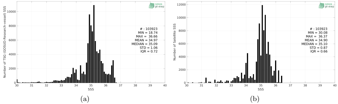
Figure 2: Histograms of SSS from TSG (GOSUD-Research-vessel) (a) and Aquarius SSS L3 OR v5 - 7-Day running (NASA-GSFC) (b) considering all match-up pairs per bins of 0.1 over the Tropical Pacific Ocean Pi-MEP region and for the full satellite product period.
