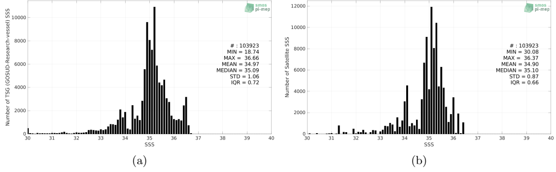
Figure 2: Histograms of SSS from TSG (GOSUD-Research-vessel) (a) and Aquarius SSS L3 OR v5 - 7-Day running (NASA-GSFC) (b) considering all match-up pairs per bins of 0.1 over the Tropical Pacific Ocean Pi-MEP region and for the full satellite product period.
