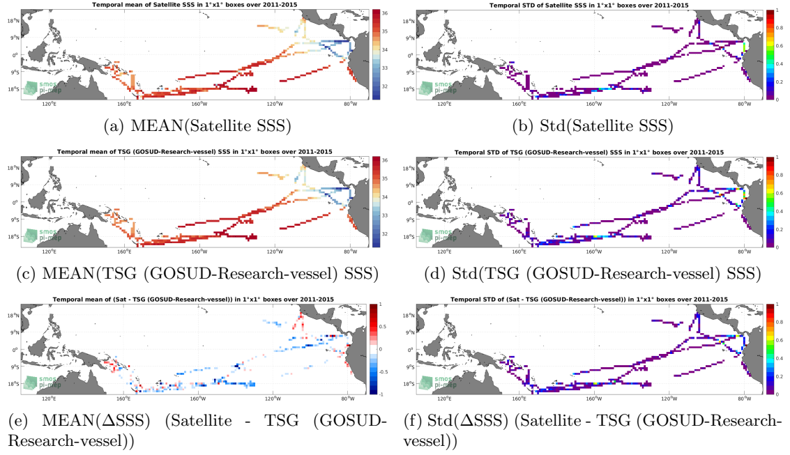
Figure 6: Temporal mean (left) and Std (right) of SSS from Aquarius SSS L3 OR v5 - 7-Day running (NASA-GSFC) (top), TSG (GOSUD-Research-vessel) (middle), and of \Delta SSS (Satellite - TSG (GOSUD-Research-vessel)). Only match-up pairs are used to generate these maps.
