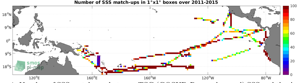
Figure 4: Number of SSS match-ups between TSG (GOSUD-Research-vessel) SSS and the Aquarius SSS L3 OR v5 - 7-Day running (NASA-GSFC) SSS product for the Tropical Pacific Ocean Pi-MEP region over 1^\circ \times 1^\circ boxes and for the full satellite product period.
