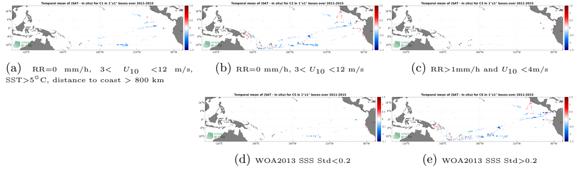
Figure 12: Temporal mean gridded over spatial boxes of size 1^\circ \times 1^\circ of \Delta SSS (Aquarius SSS L3 OR v5 - 7-Day running (NASA-GSFC) - TSG (GOSUD-Research-vessel)) for 5 different subdatasets corresponding to:RR=0 mm/h, 3 < U_{10} < 12 m/s, SST >5^\circ\text{C} , distance to coast > 800 km (a), RR=0 mm/h, 3 < U_{10} < 12 m/s (b), RR >1 mm/h and U_{10} < 4 m/s (c), WOA2013 SSS Std <0.2 (d), WOA2013 SSS Std >0.2 (e).
