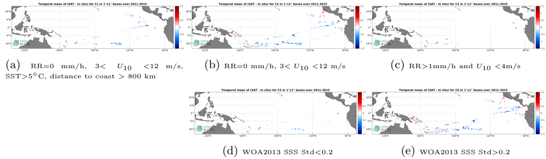
Figure 12: Temporal mean gridded over spatial boxes of size 1^\circ \times 1^\circ of \Delta SSS (Aquarius SSS L3 OR v5 - 7-Day running (NASA-GSFC) - TSG (GOSUD-Research-vessel)) for 5 different subdatasets corresponding to:RR=0 mm/h, 3 < U_{10} < 12 m/s, SST > 5^\circ\text{C} , distance to coast > 800 km (a), RR=0 mm/h, 3 < U_{10} < 12 m/s (b), RR > 1 mm/h and U_{10} < 4 m/s (c), WOA2013 SSS Std < 0.2 (d), WOA2013 SSS Std > 0.2 (e).
