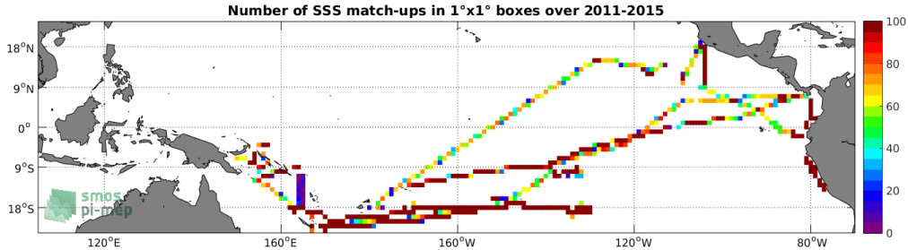
Figure 4: Number of SSS match-ups between TSG-GOSUD-Research-vessel SSS and the Aquarius-L3-OR-V5-7DAY-RUNNING-1DEG SSS product for the Tropical Pacific Ocean Pi-MEP region over 1^\circ \times 1^\circ boxes and for the full satellite product period.
