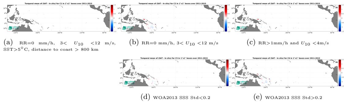
Figure 13: Temporal mean gridded over spatial boxes of size 1^\circ \times 1^\circ of \Delta SSS (Aquarius SSS L3 OR v5 - 7-Day running (NASA-GSFC) - Surface drifters) for 5 different subdatasets corresponding to: RR=0 mm/h, 3 < U_{10} < 12 m/s, SST > 5^\circ\text{C} , distance to coast > 800 km (a), RR=0 mm/h, 3 < U_{10} < 12 m/s (b), RR > 1 mm/h and U_{10} < 4 m/s (c), WOA2013 SSS Std < 0.2 (d), WOA2013 SSS Std > 0.2 (e).
