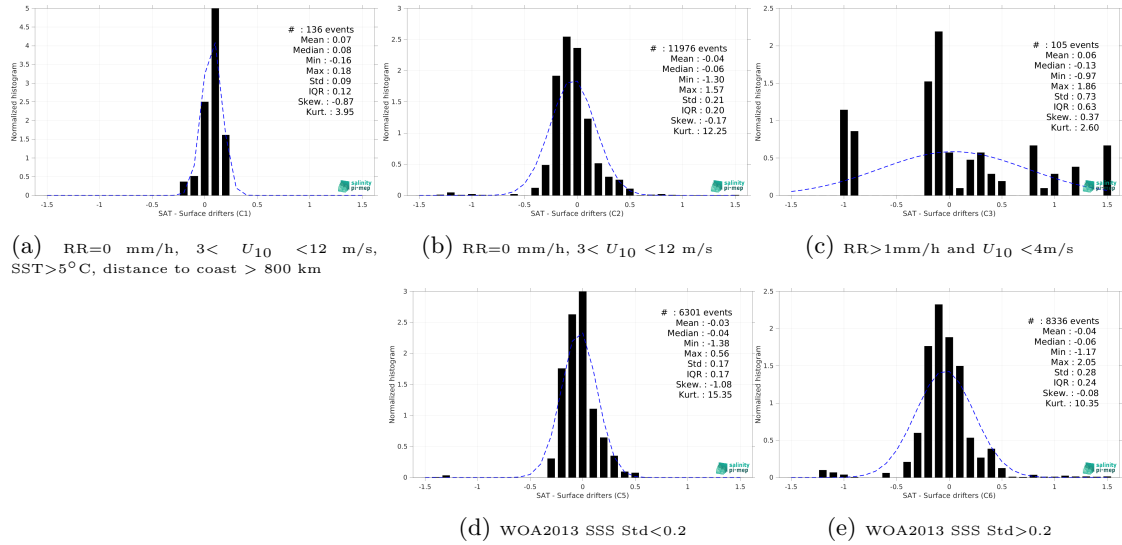
Figure 14: Normalized histogram of \Delta SSS (Aquarius SSS L3 OR v5 - 7-Day running (NASA-GSFC) - Surface drifters) for 5 different subdatasets corresponding to: RR=0 mm/h, 3 < U_{10} < 12 m/s, SST > 5°C, distance to coast > 800 km (a), RR=0 mm/h, 3 < U_{10} < 12 m/s (b), RR > 1mm/h and U_{10} < 4 m/s (c), WOA2013 SSS Std < 0.2 (d), WOA2013 SSS Std > 0.2 (e).
