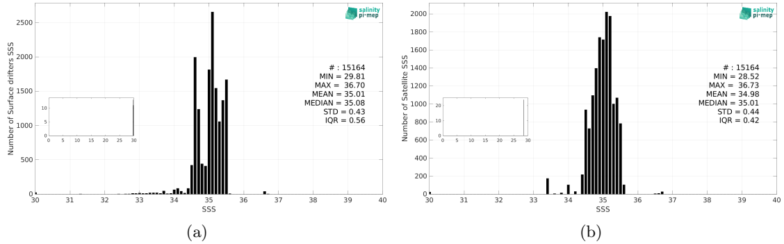
Figure 3: Histograms of SSS from Surface drifters (a) and Aquarius SSS L3 OR v5 - 7-Day running (NASA-GSFC) (b) considering all match-up pairs per bins of 0.1 over the Tropical Pacific Ocean Pi-MEP region and for the full satellite product period.
