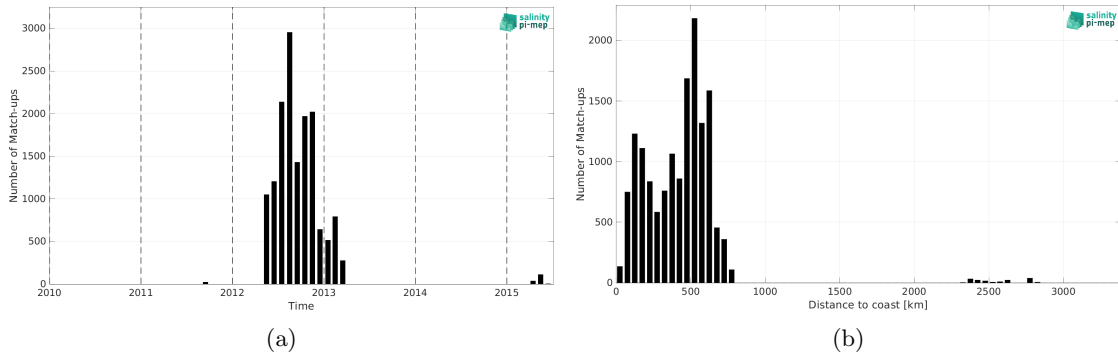
Figure 2: Number of match-ups between Surface drifters and Aquarius SSS L3 OR v5 - 7-Day running (NASA-GSFC) SSS as a function of time (a) and as function of the distance to coast (b) over the Tropical Pacific Ocean Pi-MEP region and for the full satellite product period.
