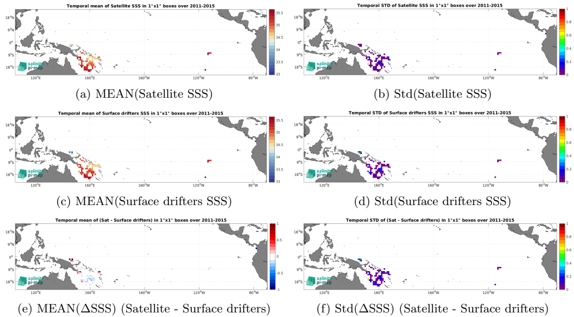
Figure 6: Temporal mean (left) and Std (right) of SSS from Aquarius SSS L3 OR v5 - 7-Day running (NASA-GSFC) (top), Surface drifters (middle), and of \Delta SSS (Satellite - Surface drifters). Only match-up pairs are used to generate these maps.
