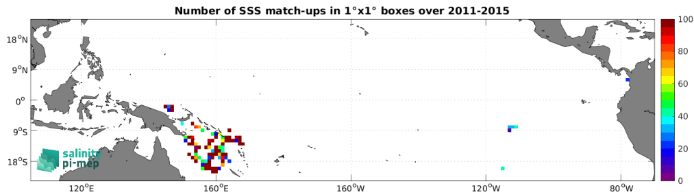
Figure 4: Number of SSS match-ups between Surface drifters SSS and the Aquarius SSS L3 OR v5 - 7-Day running (NASA-GSFC) SSS product for the Tropical Pacific Ocean Pi-MEP region over 1^\circ \times 1^\circ boxes and for the full satellite product period.
