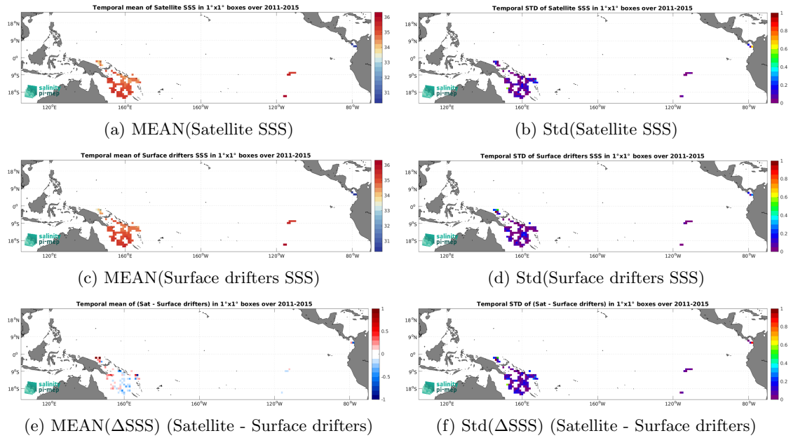
Figure 5: Temporal mean (left) and Std (right) of SSS from Aquarius SSS L3 OR v5 - 7-Day running (NASA-GSFC) (top), Surface drifters (middle), and of \Delta SSS (Satellite - Surface drifters). Only match-up pairs are used to generate these maps.
