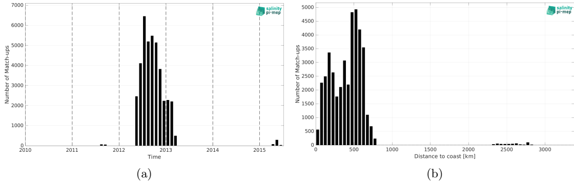
Figure 1: Number of match-ups between Surface drifters and Aquarius SSS L3 OR v5 - 7-Day running (NASA-GSFC) SSS as a function of time (a) and as function of the distance to coast (b) over the Tropical Pacific Ocean Pi-MEP region and for the full satellite product period.
