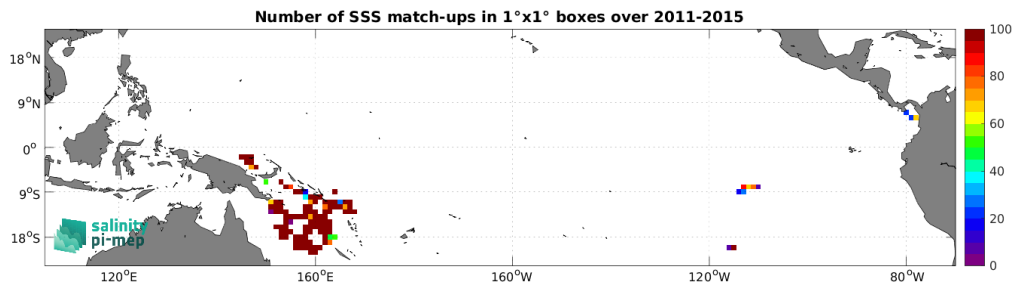
Figure 3: Number of SSS match-ups between Surface drifters SSS and the Aquarius SSS L3 OR v5 - 7-Day running (NASA-GSFC) SSS product for the Tropical Pacific Ocean Pi-MEP region over 1^\circ \times 1^\circ boxes and for the full satellite product period.
