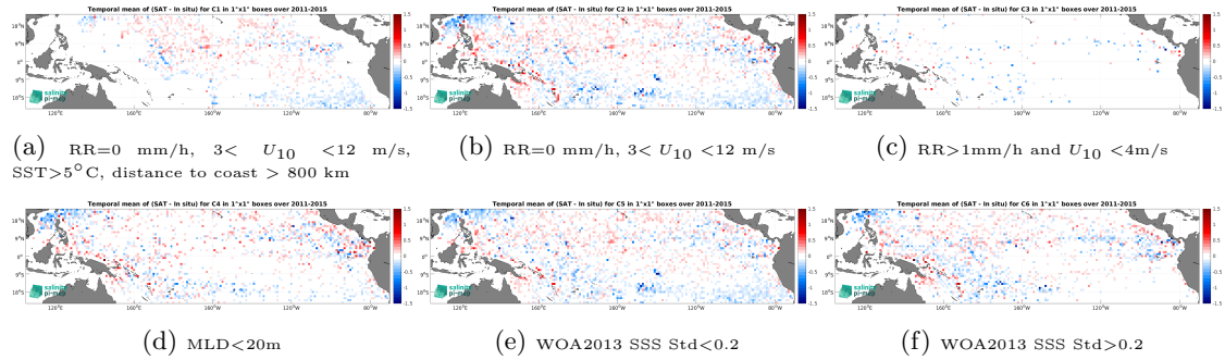
Figure 14: Temporal mean gridded over spatial boxes of size 1^\circ \times 1^\circ of \Delta SSS (Aquarius SSS L3 OR v5 - 7-Day running (NASA-GSFC) - Argo) for 6 different subdatasets corresponding to: RR=0 mm/h, 3 < U_{10} < 12 m/s, SST > 5°C, distance to coast > 800 km (a), RR=0 mm/h, 3 < U_{10} < 12 m/s (b), RR > 1mm/h and U_{10} < 4 m/s (c),MLD < 20m (d),WOA2013 SSS Std < 0.2 (e),WOA2013 SSS Std > 0.2 (f).
