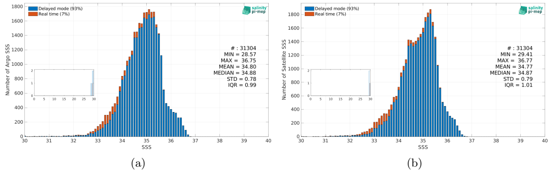
Figure 3: Histograms of SSS from Argo (a) and Aquarius SSS L3 OR v5 - 7-Day running (NASA-GSFC) (b) considering all match-up pairs per bins of 0.1 over the Tropical Pacific Ocean Pi-MEP region and for the full satellite product period.
