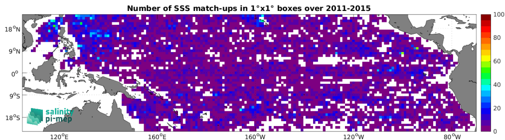
Figure 5: Number of SSS match-ups between Argo SSS and the Aquarius SSS L3 OR v5 - 7-Day running (NASA-GSFC) SSS product for the Tropical Pacific Ocean Pi-MEP region over 1^\circ \times 1^\circ boxes and for the full satellite product period.
