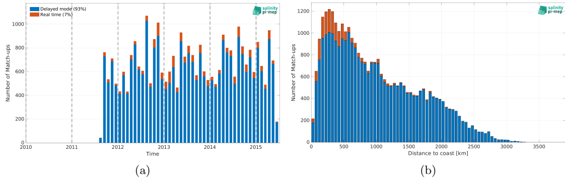
Figure 2: Number of match-ups between Argo and Aquarius SSS L3 OR v5 - 7-Day running (NASA-GSFC) SSS as a function of time (a) and as function of the distance to coast (b) over the Tropical Pacific Ocean Pi-MEP region and for the full satellite product period.
