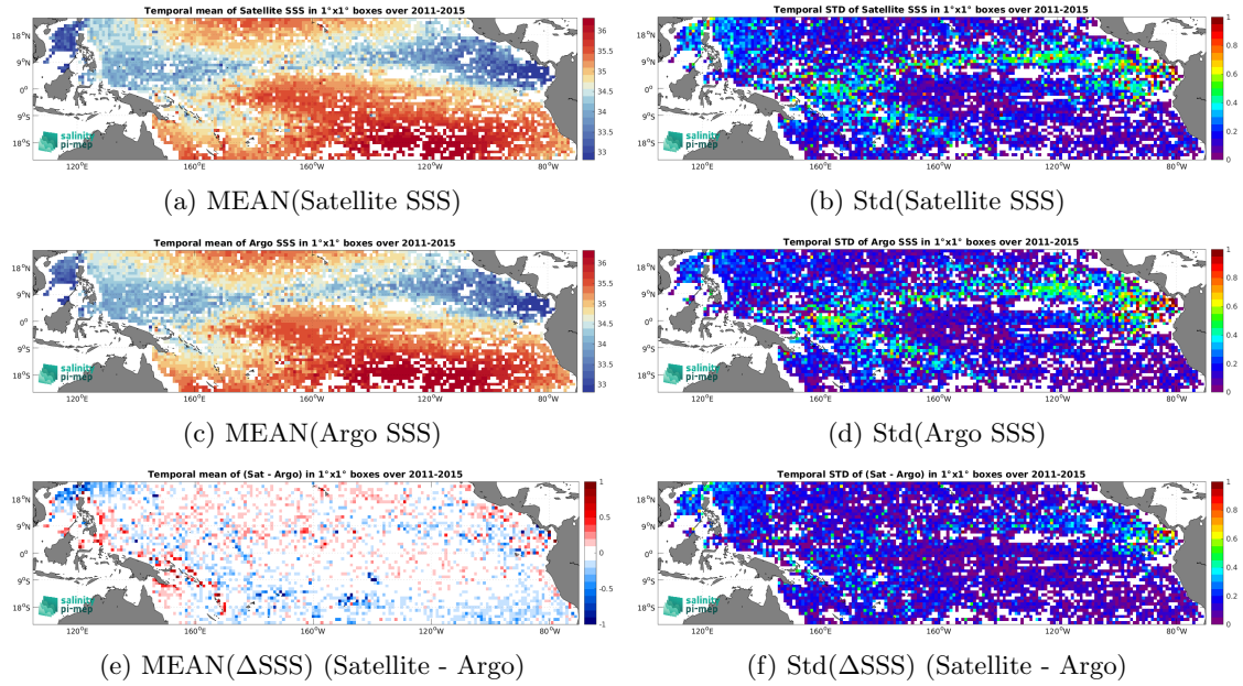
Figure 7: Temporal mean (left) and Std (right) of SSS from Aquarius SSS L3 OR v5 - 7-Day running (NASA-GSFC) (top), Argo (middle), and of \Delta SSS (Satellite - Argo). Only match-up pairs are used to generate these maps.
