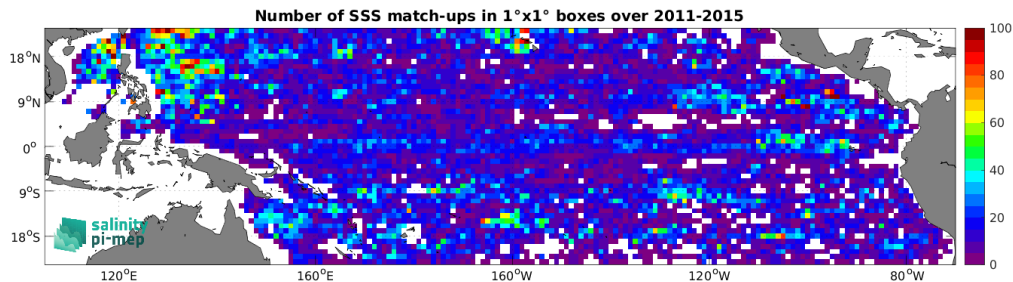
Figure 4: Number of SSS match-ups between Argo SSS and the Aquarius SSS L3 OR v5 - 7-Day running (NASA-GSFC) SSS product for the Tropical Pacific Ocean Pi-MEP region over 1^\circ \times 1^\circ boxes and for the full satellite product period.
