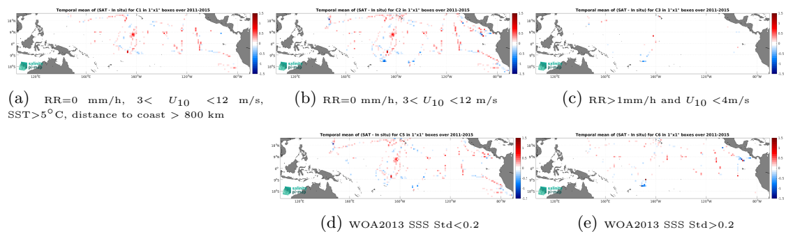
Figure 14: Temporal mean gridded over spatial boxes of size 1^\circ \times 1^\circ of \Delta\text{SSS} (Aquarius SSS L3 OR v5 - 7-Day running - Rain mask (NASA-GSFC) - TSG (SAMOS)) for 5 different subdatasets corresponding to: RR=0 mm/h, 3 < U_{10} < 12 m/s, SST > 5°C, distance to coast > 800 km (a), RR=0 mm/h, 3 < U_{10} < 12 m/s (b), RR > 1mm/h and U_{10} < 4 m/s (c), WOA2013 SSS Std < 0.2 (d), WOA2013 SSS Std > 0.2 (e).
