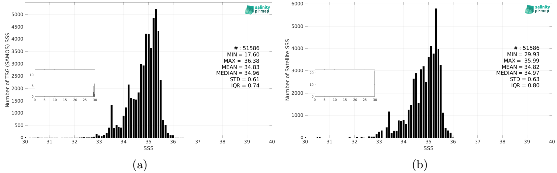
Figure 3: Histograms of SSS from TSG (SAMOS) (a) and Aquarius SSS L3 OR v5 - 7-Day running - Rain mask (NASA-GSFC) (b) considering all match-up pairs per bins of 0.1 over the Tropical Pacific Ocean Pi-MEP region and for the full satellite product period.
