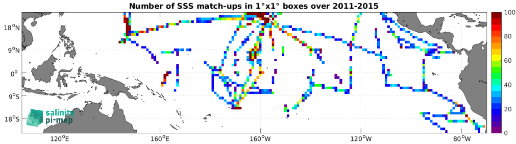
Figure 5: Number of SSS match-ups between TSG (SAMOS) SSS and the Aquarius SSS L3 OR v5 - 7-Day running - Rain mask (NASA-GSFC) SSS product for the Tropical Pacific Ocean Pi-MEP region over 1^\circ \times 1^\circ boxes and for the full satellite product period.
