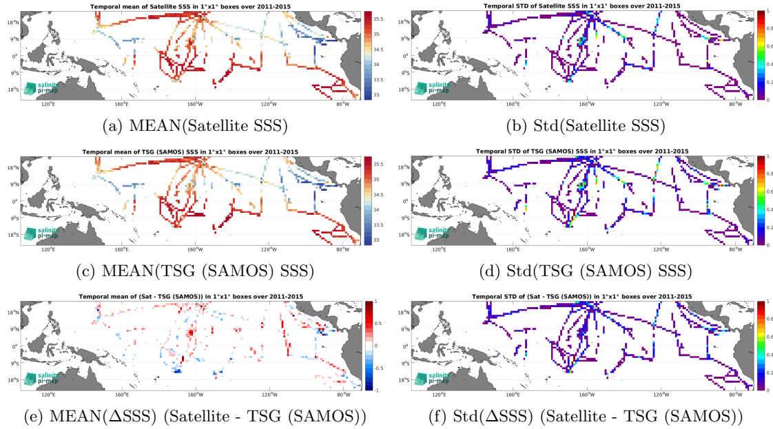
Figure 7: Temporal mean (left) and Std (right) of SSS from Aquarius SSS L3 OR v5 - 7-Day running - Rain mask (NASA-GSFC) (top), TSG (SAMOS) (middle), and of \Delta SSS (Satellite - TSG (SAMOS)). Only match-up pairs are used to generate these maps.
