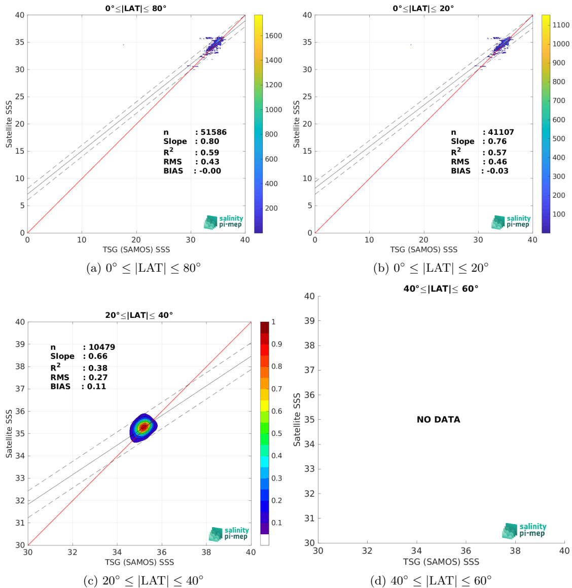
Figure 10: Contour maps of the concentration of Aquarius SSS L3 OR v5 - 7-Day running - Rain mask (NASA-GSFC) SSS (y-axis) versus TSG (SAMOS) SSS (x-axis) at match-up pairs for different latitude bands. For each plot, the red line shows x=y . The black thin and dashed lines indicate a linear fit through the data cloud and the \pm 95\% confidence levels, respectively. The number match-up pairs n , the slope and R^2 coefficient of the linear fit, the root mean square (RMS) and the mean bias between satellite and in situ data are indicated for each latitude band in each plots.
