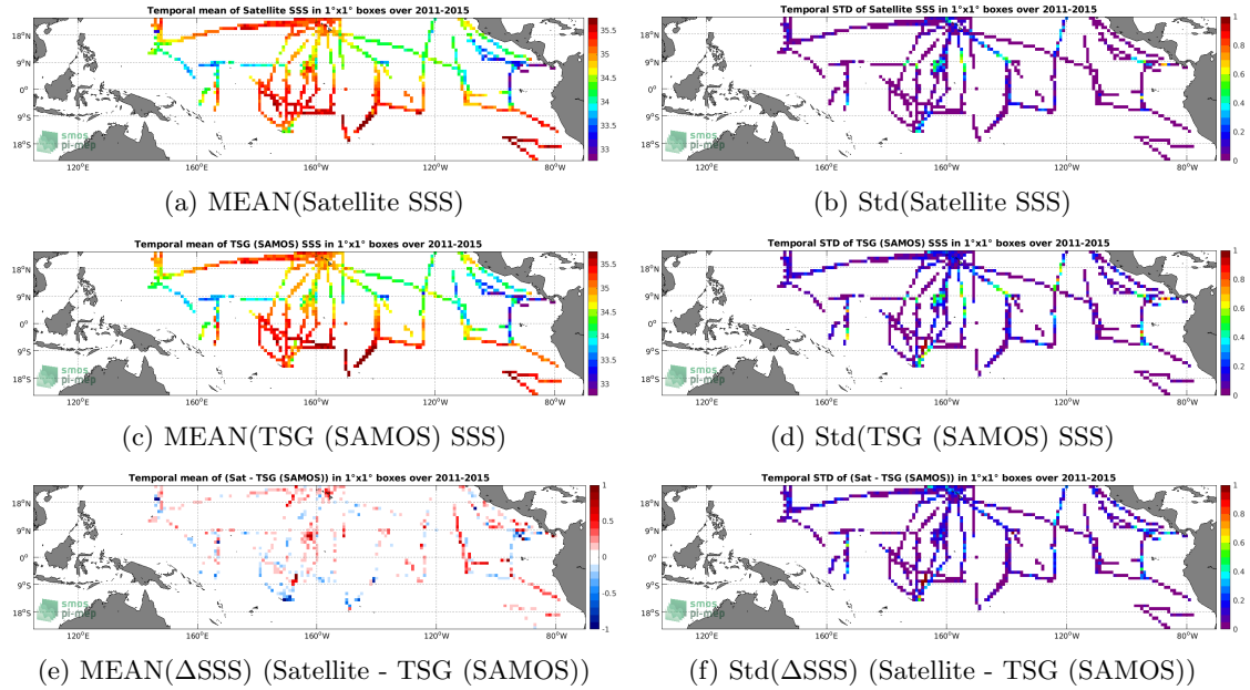
Figure 6: Temporal mean (left) and Std (right) of SSS from Aquarius SSS L3 OR v5 - 7-Day running - Rain mask (NASA-GSFC) (top), TSG (SAMOS) (middle), and of \Delta SSS (Satellite - TSG (SAMOS)). Only match-up pairs are used to generate these maps.
