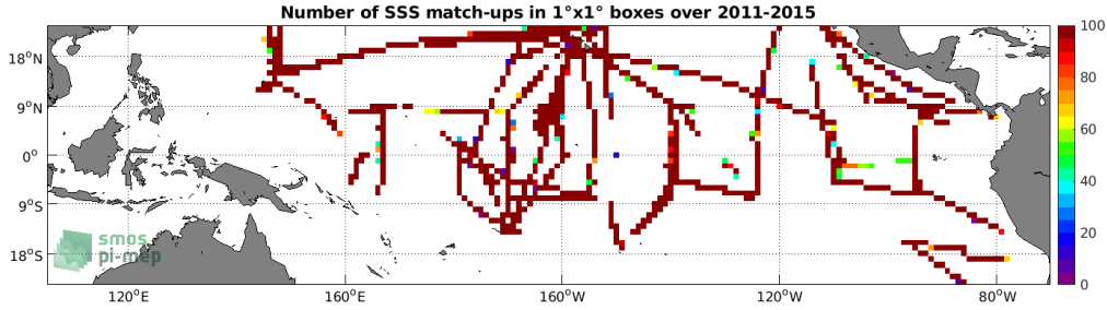
Figure 4: Number of SSS match-ups between TSG (SAMOS) SSS and the Aquarius SSS L3 OR v5 - 7-Day running - Rain mask (NASA-GSFC) SSS product for the Tropical Pacific Ocean Pi-MEP region over 1^\circ \times 1^\circ boxes and for the full satellite product period.
