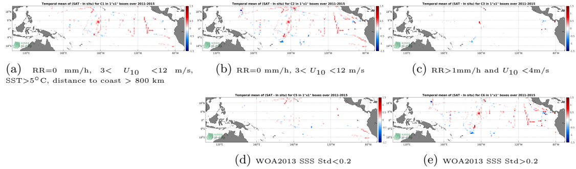
Figure 12: Temporal mean gridded over spatial boxes of size 1^{\circ}\times 1^{\circ} of \Delta\text{SSS} (Aquarius SSS L3 OR v5 - 7-Day running - Rain mask (NASA-GSFC) - TSG (SAMOS)) for 5 different subdatasets corresponding to:RR=0 mm/h, 3 < U_{10} < 12 m/s, SST >5^{\circ}\text{C} , distance to coast > 800 km (a), RR=0 mm/h, 3 < U_{10} < 12 m/s (b), RR >1 mm/h and U_{10} < 4 m/s (c), WOA2013 SSS Std <0.2 (d), WOA2013 SSS Std >0.2 (e).
