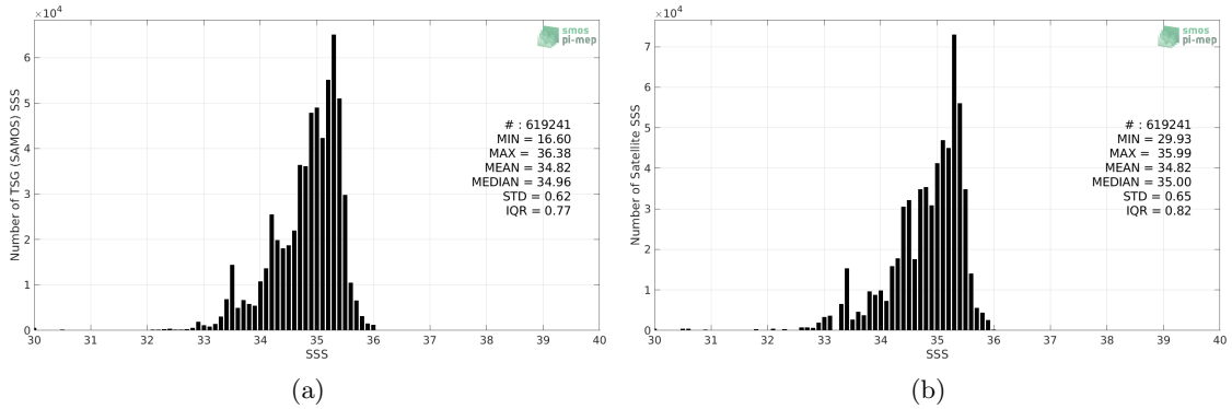
Figure 2: Histograms of SSS from TSG (SAMOS) (a) and Aquarius SSS L3 OR v5 - 7-Day running - Rain mask (NASA-GSFC) (b) considering all match-up pairs per bins of 0.1 over the Tropical Pacific Ocean Pi-MEP region and for the full satellite product period.
