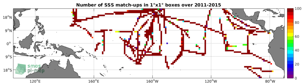
Figure 4: Number of SSS match-ups between TSG-SAMOS SSS and the Aquarius-L3-OR-V5-7DAY-RUNNING-RAIN-MASK-1DEG SSS product for the Tropical Pacific Ocean Pi-MEP region over 1^\circ \times 1^\circ boxes and for the full satellite product period.
