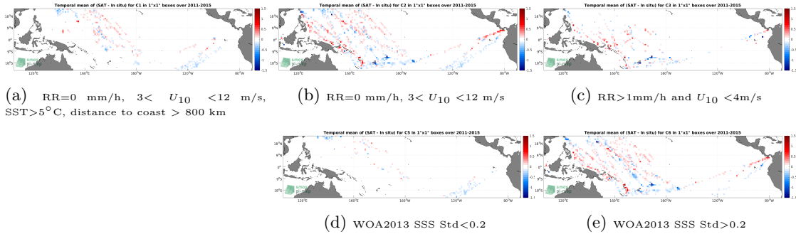
Figure 12: Temporal mean gridded over spatial boxes of size 1^{\circ}\times 1^{\circ} of \Delta\text{SSS} (Aquarius SSS L3 OR v5 - 7-Day running - Rain mask (NASA-GSFC) - TSG (LEGOS-DM)) for 5 different subdatasets corresponding to:RR=0 mm/h, 3 < U_{10} < 12 m/s, SST >5^{\circ}\text{C} , distance to coast > 800 km (a), RR=0 mm/h, 3 < U_{10} < 12 m/s (b), RR >1 mm/h and U_{10} < 4 m/s (c), WOA2013 SSS Std <0.2 (d), WOA2013 SSS Std >0.2 (e).
