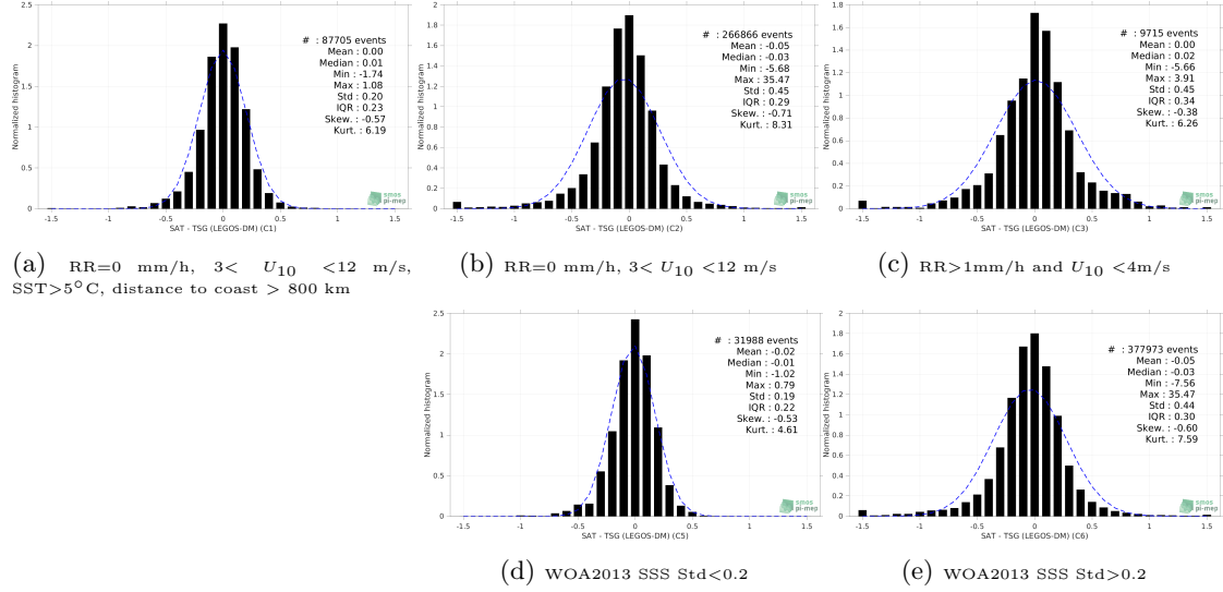
Figure 13: Normalized histogram of \Delta\text{SSS} (Aquarius SSS L3 OR v5 - 7-Day running - Rain mask (NASA-GSFC) - TSG (LEGOS-DM)) for 5 different subdatasets corresponding to: RR=0 mm/h, 3 < U_{10} < 12 m/s, SST>5°C, distance to coast > 800 km (a), RR=0 mm/h, 3 < U_{10} < 12 m/s (b), RR>1mm/h and U_{10} < 4 m/s (c), WOA2013 SSS Std<0.2 (d), WOA2013 SSS Std>0.2 (e).
