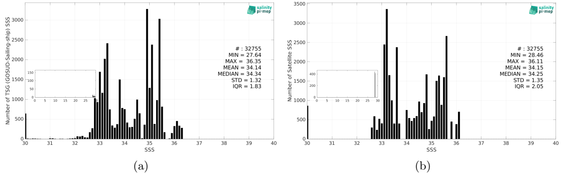
Figure 3: Histograms of SSS from TSG (GOSUD-Sailing-ship) (a) and Aquarius SSS L3 OR v5 - 7-Day running - Rain mask (NASA-GSFC) (b) considering all match-up pairs per bins of 0.1 over the Tropical Pacific Ocean Pi-MEP region and for the full satellite product period.
