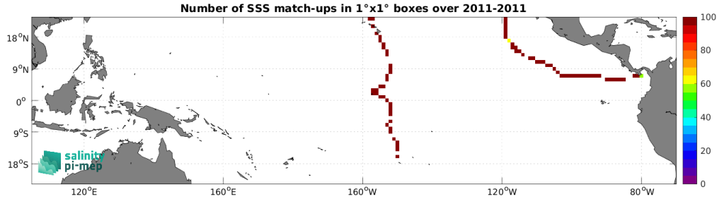
Figure 5: Number of SSS match-ups between TSG (GOSUD-Sailing-ship) SSS and the Aquarius SSS L3 OR v5 - 7-Day running - Rain mask (NASA-GSFC) SSS product for the Tropical Pacific Ocean Pi-MEP region over 1^\circ \times 1^\circ boxes and for the full satellite product period.
