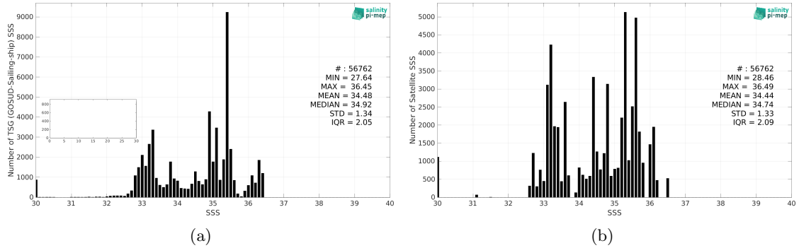
Figure 2: Histograms of SSS from TSG (GOSUD-Sailing-ship) (a) and Aquarius SSS L3 OR v5 - 7-Day running - Rain mask (NASA-GSFC) (b) considering all match-up pairs per bins of 0.1 over the Tropical Pacific Ocean Pi-MEP region and for the full satellite product period.
