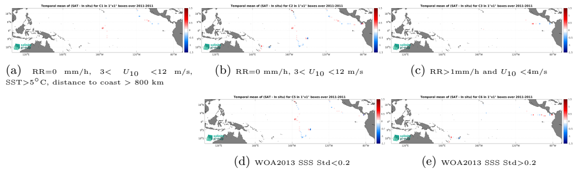
Figure 12: Temporal mean gridded over spatial boxes of size 1^{\circ}\times 1^{\circ} of \Delta SSS (Aquarius SSS L3 OR v5 - 7-Day running - Rain mask (NASA-GSFC) - TSG (GOSUD-Sailing-ship)) for 5 different subdatasets corresponding to:RR=0 mm/h, 3 < U_{10} < 12 m/s, SST >5^{\circ}\text{C} , distance to coast > 800 km (a), RR=0 mm/h, 3 < U_{10} < 12 m/s (b), RR >1 mm/h and U_{10} < 4 m/s (c), WOA2013 SSS Std <0.2 (d), WOA2013 SSS Std >0.2 (e).
