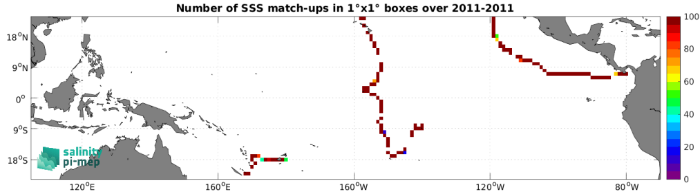
Figure 4: Number of SSS match-ups between TSG (GOSUD-Sailing-ship) SSS and the Aquarius SSS L3 OR v5 - 7-Day running - Rain mask (NASA-GSFC) SSS product for the Tropical Pacific Ocean Pi-MEP region over 1^\circ \times 1^\circ boxes and for the full satellite product period.
