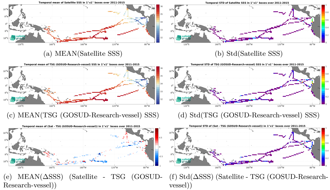
Figure 7: Temporal mean (left) and Std (right) of SSS from Aquarius SSS L3 OR v5 - 7-Day running - Rain mask (NASA-GSFC) (top), TSG (GOSUD-Research-vessel) (middle), and of \Delta SSS (Satellite - TSG (GOSUD-Research-vessel)). Only match-up pairs are used to generate these maps.
