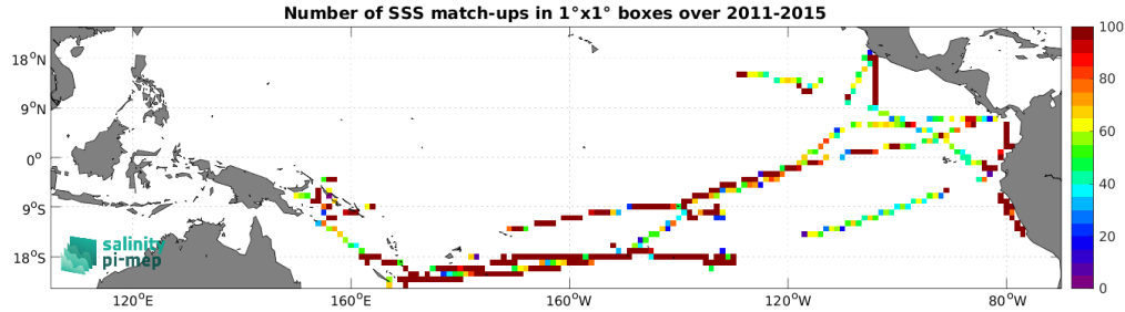
Figure 5: Number of SSS match-ups between TSG (GOSUD-Research-vessel) SSS and the Aquarius SSS L3 OR v5 - 7-Day running - Rain mask (NASA-GSFC) SSS product for the Tropical Pacific Ocean Pi-MEP region over 1^\circ \times 1^\circ boxes and for the full satellite product period.
