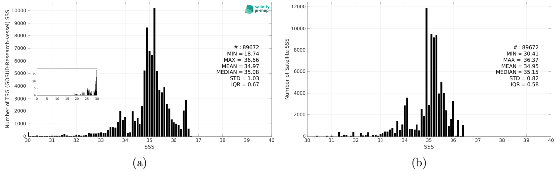
Figure 3: Histograms of SSS from TSG (GOSUD-Research-vessel) (a) and Aquarius SSS L3 OR v5 - 7-Day running - Rain mask (NASA-GSFC) (b) considering all match-up pairs per bins of 0.1 over the Tropical Pacific Ocean Pi-MEP region and for the full satellite product period.
