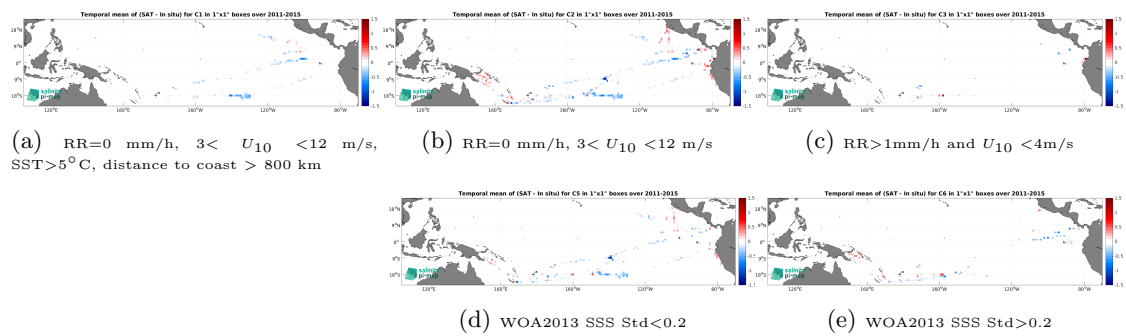
Figure 14: Temporal mean gridded over spatial boxes of size 1^\circ \times 1^\circ of \Delta SSS (Aquarius SSS L3 OR v5 - 7-Day running - Rain mask (NASA-GSFC) - TSG (GOSUD-Research-vessel)) for 5 different subdatasets corresponding to:RR=0 mm/h, 3 < U_{10} < 12 m/s, SST > 5^\circ\text{C} , distance to coast > 800 km (a), RR=0 mm/h, 3 < U_{10} < 12 m/s (b), RR > 1 mm/h and U_{10} < 4 m/s (c), WOA2013 SSS Std < 0.2 (d), WOA2013 SSS Std > 0.2 (e).
