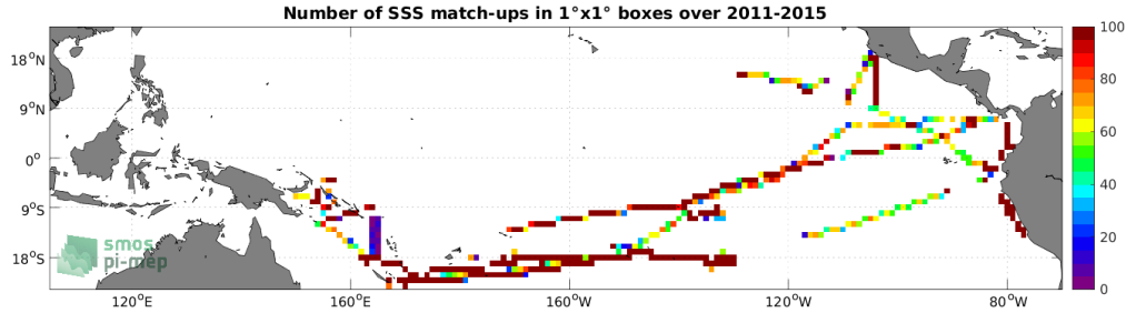
Figure 4: Number of SSS match-ups between TSG (GOSUD-Research-vessel) SSS and the Aquarius SSS L3 OR v5 - 7-Day running - Rain mask (NASA-GSFC) SSS product for the Tropical Pacific Ocean Pi-MEP region over 1^\circ \times 1^\circ boxes and for the full satellite product period.
