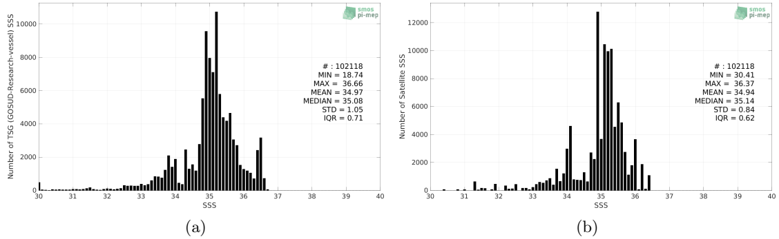
Figure 2: Histograms of SSS from TSG (GOSUD-Research-vessel) (a) and Aquarius SSS L3 OR v5 - 7-Day running - Rain mask (NASA-GSFC) (b) considering all match-up pairs per bins of 0.1 over the Tropical Pacific Ocean Pi-MEP region and for the full satellite product period.
