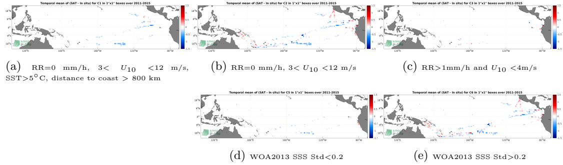
Figure 12: Temporal mean gridded over spatial boxes of size 1^{\circ}\times 1^{\circ} of \Delta SSS (Aquarius SSS L3 OR v5 - 7-Day running - Rain mask (NASA-GSFC) - TSG (GOSUD-Research-vessel)) for 5 different subdatasets corresponding to:RR=0 mm/h, 3 < U_{10} < 12 m/s, SST >5^{\circ}\text{C} , distance to coast > 800 km (a), RR=0 mm/h, 3 < U_{10} < 12 m/s (b), RR >1 mm/h and U_{10} < 4 m/s (c), WOA2013 SSS Std <0.2 (d), WOA2013 SSS Std >0.2 (e).
