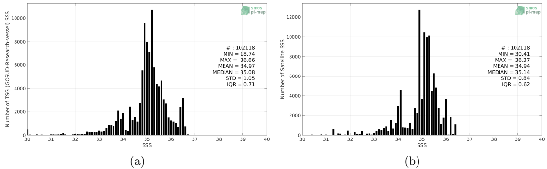
Figure 2: Histograms of SSS from TSG (GOSUD-Research-vessel) (a) and Aquarius SSS L3 OR v5 - 7-Day running - Rain mask (NASA-GSFC) (b) considering all match-up pairs per bins of 0.1 over the Tropical Pacific Ocean Pi-MEP region and for the full satellite product period.
