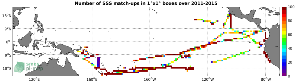
Figure 4: Number of SSS match-ups between TSG (GOSUD-Research-vessel) SSS and the Aquarius SSS L3 OR v5 - 7-Day running - Rain mask (NASA-GSFC) SSS product for the Tropical Pacific Ocean Pi-MEP region over 1^\circ \times 1^\circ boxes and for the full satellite product period.
