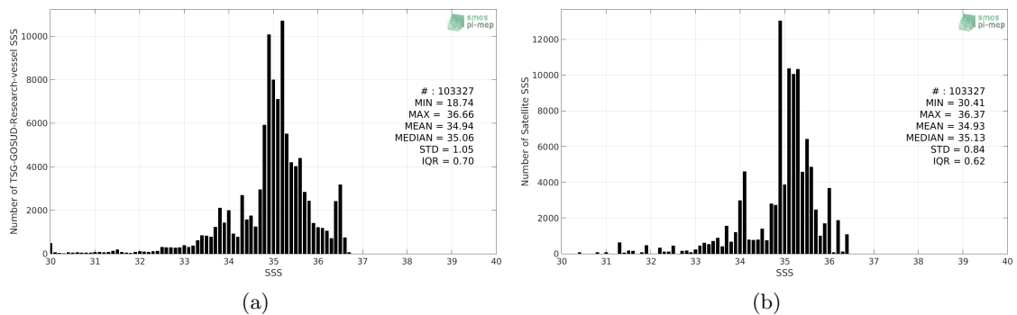
Figure 2: Histograms of SSS from TSG-GOSUD-Research-vessel (a) and Aquarius-L3-OR-V5-7DAY-RUNNING-RAIN-MASK-1DEG (b) considering all match-up pairs per bins of 0.1 over the Tropical Pacific Ocean Pi-MEP region and for the full satellite product period.
