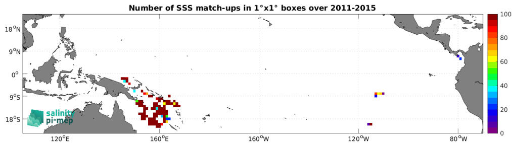
Figure 4: Number of SSS match-ups between Surface drifters SSS and the Aquarius SSS L3 OR v5 - 7-Day running - Rain mask (NASA-GSFC) SSS product for the Tropical Pacific Ocean Pi-MEP region over 1^\circ \times 1^\circ boxes and for the full satellite product period.
