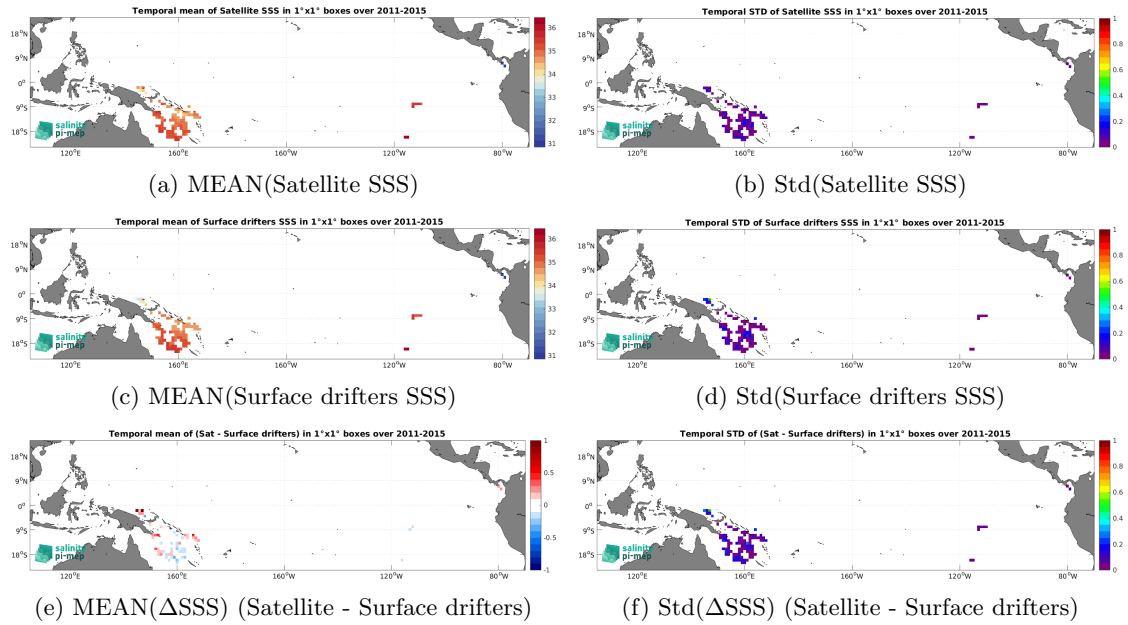
Figure 6: Temporal mean (left) and Std (right) of SSS from Aquarius SSS L3 OR v5 - 7-Day running - Rain mask (NASA-GSFC) (top), Surface drifters (middle), and of \Delta SSS (Satellite - Surface drifters). Only match-up pairs are used to generate these maps.
