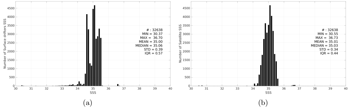
Figure 3: Histograms of SSS from Surface drifters (a) and Aquarius SSS L3 OR v5 - 7-Day running - Rain mask (NASA-GSFC) (b) considering all match-up pairs per bins of 0.1 over the Tropical Pacific Ocean Pi-MEP region and for the full satellite product period.
