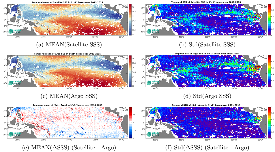
Figure 7: Temporal mean (left) and Std (right) of SSS from Aquarius SSS L3 OR v5 - 7-Day running - Rain mask (NASA-GSFC) (top), Argo (middle), and of \Delta SSS (Satellite - Argo). Only match-up pairs are used to generate these maps.
