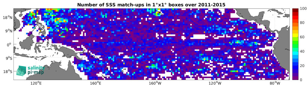
Figure 5: Number of SSS match-ups between Argo SSS and the Aquarius SSS L3 OR v5 - 7-Day running - Rain mask (NASA-GSFC) SSS product for the Tropical Pacific Ocean Pi-MEP region over 1^\circ \times 1^\circ boxes and for the full satellite product period.
