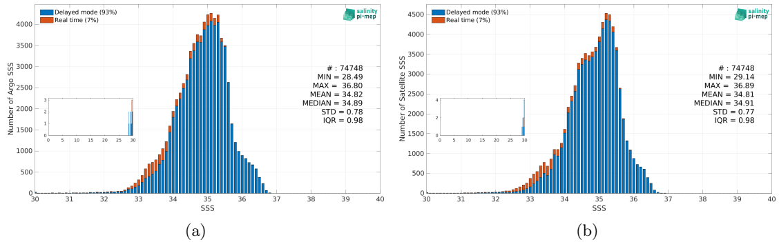
Figure 3: Histograms of SSS from Argo (a) and Aquarius SSS L3 OR v5 - 7-Day running - Rain mask (NASA-GSFC) (b) considering all match-up pairs per bins of 0.1 over the Tropical Pacific Ocean Pi-MEP region and for the full satellite product period.
