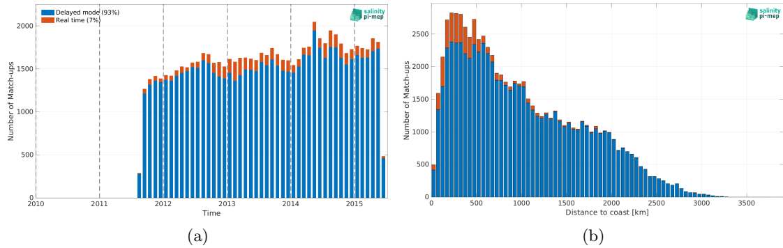
Figure 2: Number of match-ups between Argo and Aquarius SSS L3 OR v5 - 7-Day running - Rain mask (NASA-GSFC) SSS as a function of time (a) and as function of the distance to coast (b) over the Tropical Pacific Ocean Pi-MEP region and for the full satellite product period.
