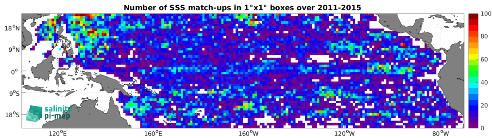
Figure 4: Number of SSS match-ups between Argo SSS and the Aquarius SSS L3 OR v5 - 7-Day running - Rain mask (NASA-GSFC) SSS product for the Tropical Pacific Ocean Pi-MEP region over 1^\circ \times 1^\circ boxes and for the full satellite product period.
