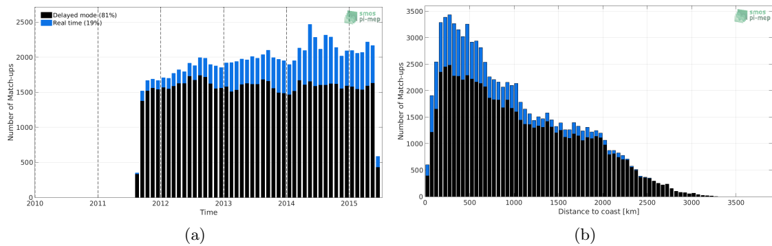
Figure 1: Number of match-ups between Argo and Aquarius-L3-OR-V5-7DAY-RUNNING-RAIN-MASK-1DEG SSS as a function of time (a) and as function of the distance to coast (b) over the Tropical Pacific Ocean Pi-MEP region and for the full satellite product period.
