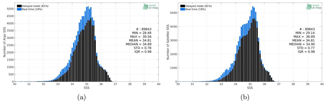
Figure 2: Histograms of SSS from Argo (a) and Aquarius-L3-OR-V5-7DAY-RUNNING-RAIN-MASK-1DEG (b) considering all match-up pairs per bins of 0.1 over the Tropical Pacific Ocean Pi-MEP region and for the full satellite product period.
