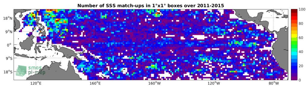
Figure 4: Number of SSS match-ups between Argo SSS and the Aquarius-L3-OR-V5-7DAY-RUNNING-RAIN-MASK-1DEG SSS product for the Tropical Pacific Ocean Pi-MEP region over 1^\circ \times 1^\circ boxes and for the full satellite product period.
