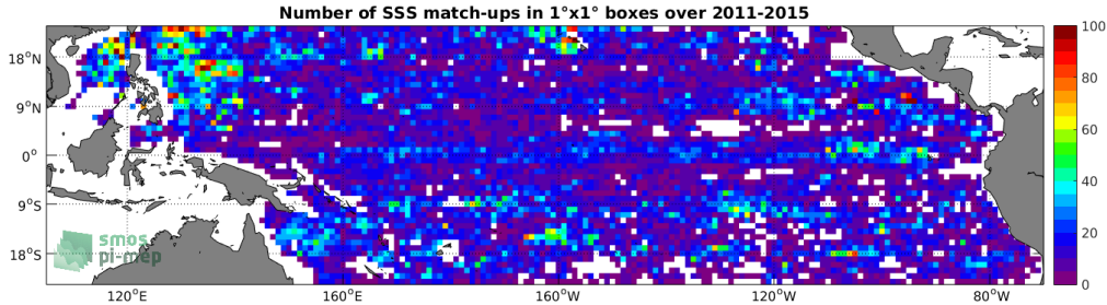
Figure 4: Number of SSS match-ups between Argo SSS and the Aquarius-L3-OR-V5-7DAY-RUNNING-RAIN-MASK-1DEG SSS product for the Tropical Pacific Ocean Pi-MEP region over 1^\circ \times 1^\circ boxes and for the full satellite product period.
