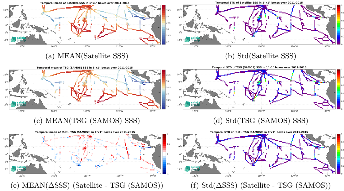
Figure 7: Temporal mean (left) and Std (right) of SSS from Aquarius SSS L3 OR v5 - Monthly (NASA-GSFC) (top), TSG (SAMOS) (middle), and of \Delta SSS (Satellite - TSG (SAMOS)). Only match-up pairs are used to generate these maps.
