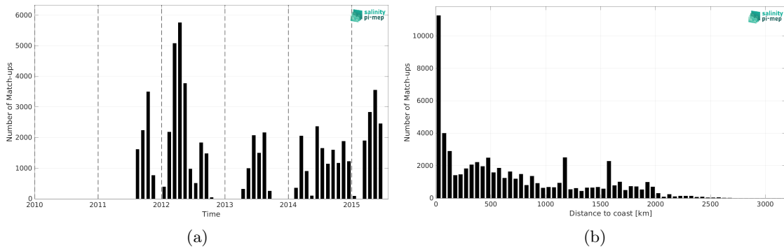
Figure 2: Number of match-ups between TSG (SAMOS) and Aquarius SSS L3 OR v5 - Monthly (NASA-GSFC) SSS as a function of time (a) and as function of the distance to coast (b) over the Tropical Pacific Ocean Pi-MEP region and for the full satellite product period.
