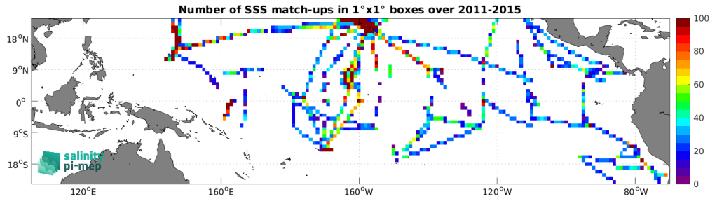
Figure 5: Number of SSS match-ups between TSG (SAMOS) SSS and the Aquarius SSS L3 OR v5 - Monthly (NASA-GSFC) SSS product for the Tropical Pacific Ocean Pi-MEP region over 1^\circ \times 1^\circ boxes and for the full satellite product period.
