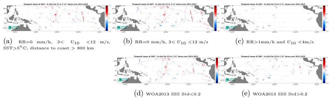
Figure 14: Temporal mean gridded over spatial boxes of size 1^\circ \times 1^\circ of \Delta SSS (Aquarius SSS L3 OR v5 - Monthly (NASA-GSFC) - TSG (SAMOS)) for 5 different subdatasets corresponding to:RR=0 mm/h, 3 < U_{10} < 12 m/s, SST > 5^\circ\text{C} , distance to coast > 800 km (a), RR=0 mm/h, 3 < U_{10} < 12 m/s (b), RR > 1 mm/h and U_{10} < 4 m/s (c), WOA2013 SSS Std < 0.2 (d), WOA2013 SSS Std > 0.2 (e).
