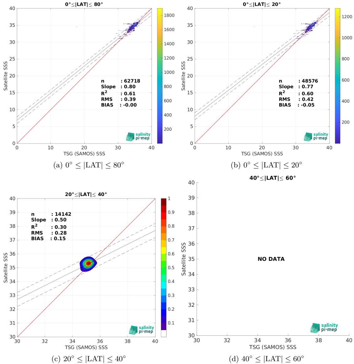
Figure 10: Contour maps of the concentration of Aquarius SSS L3 OR v5 - Monthly (NASA-GSFC) SSS (y-axis) versus TSG (SAMOS) SSS (x-axis) at match-up pairs for different latitude bands. For each plot, the red line shows x=y . The black thin and dashed lines indicate a linear fit through the data cloud and the \pm 95\% confidence levels, respectively. The number match-up pairs n , the slope and R^2 coefficient of the linear fit, the root mean square (RMS) and the mean bias between satellite and in situ data are indicated for each latitude band in each plots.
