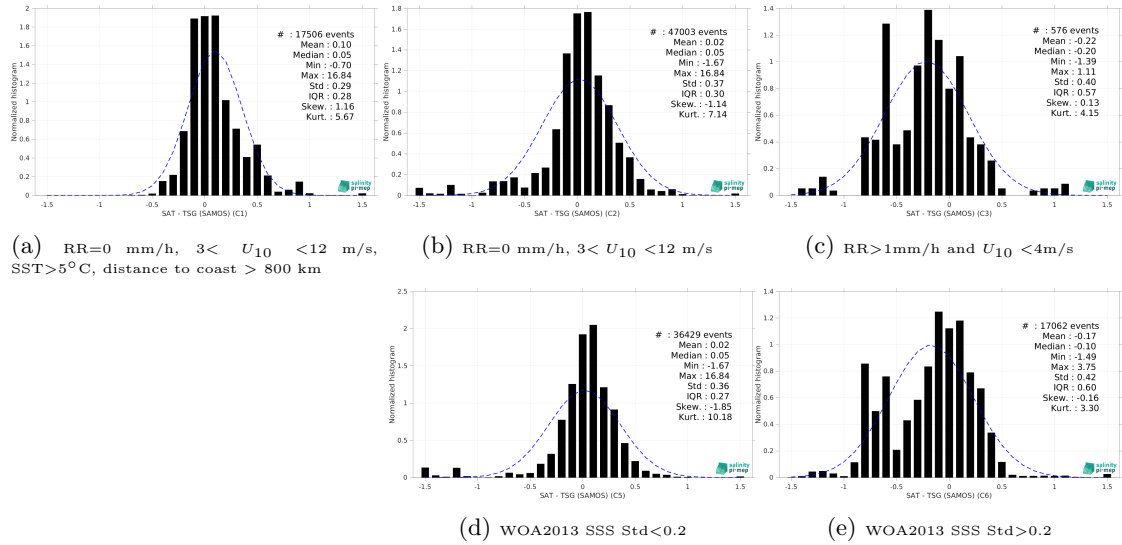
Figure 15: Normalized histogram of \Delta SSS (Aquarius SSS L3 OR v5 - Monthly (NASA-GSFC) - TSG (SAMOS)) for 5 different subdatasets corresponding to: RR=0 mm/h, 3 < U_{10} < 12 m/s, SST > 5°C, distance to coast > 800 km (a), RR=0 mm/h, 3 < U_{10} < 12 m/s (b), RR > 1mm/h and U_{10} < 4 m/s (c), WOA2013 SSS Std < 0.2 (d), WOA2013 SSS Std > 0.2 (e).
