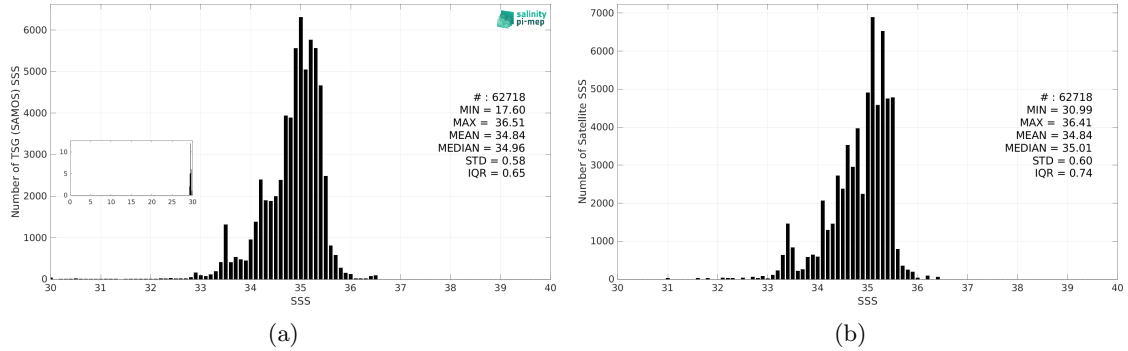
Figure 3: Histograms of SSS from TSG (SAMOS) (a) and Aquarius SSS L3 OR v5 - Monthly (NASA-GSFC) (b) considering all match-up pairs per bins of 0.1 over the Tropical Pacific Ocean Pi-MEP region and for the full satellite product period.
