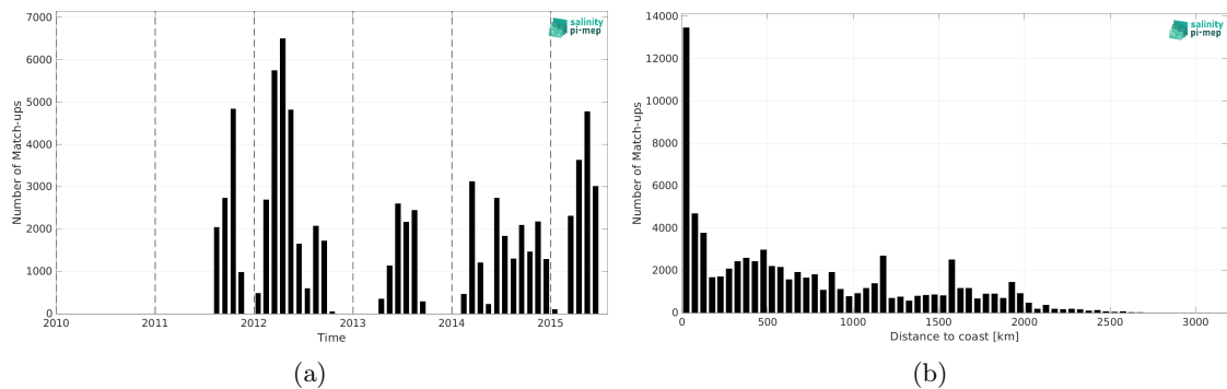
Figure 1: Number of match-ups between TSG (SAMOS) and Aquarius SSS L3 OR v5 - Monthly (NASA-GSFC) SSS as a function of time (a) and as function of the distance to coast (b) over the Tropical Pacific Ocean Pi-MEP region and for the full satellite product period.
