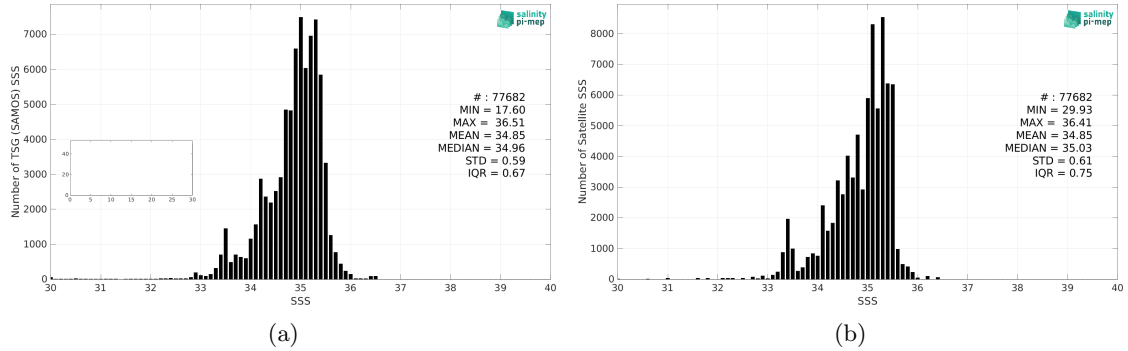
Figure 2: Histograms of SSS from TSG (SAMOS) (a) and Aquarius SSS L3 OR v5 - Monthly (NASA-GSFC) (b) considering all match-up pairs per bins of 0.1 over the Tropical Pacific Ocean Pi-MEP region and for the full satellite product period.
