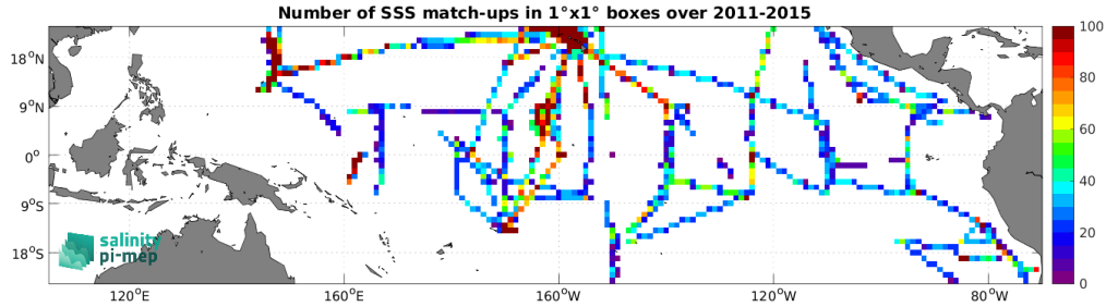
Figure 4: Number of SSS match-ups between TSG (SAMOS) SSS and the Aquarius SSS L3 OR v5 - Monthly (NASA-GSFC) SSS product for the Tropical Pacific Ocean Pi-MEP region over 1^\circ \times 1^\circ boxes and for the full satellite product period.
