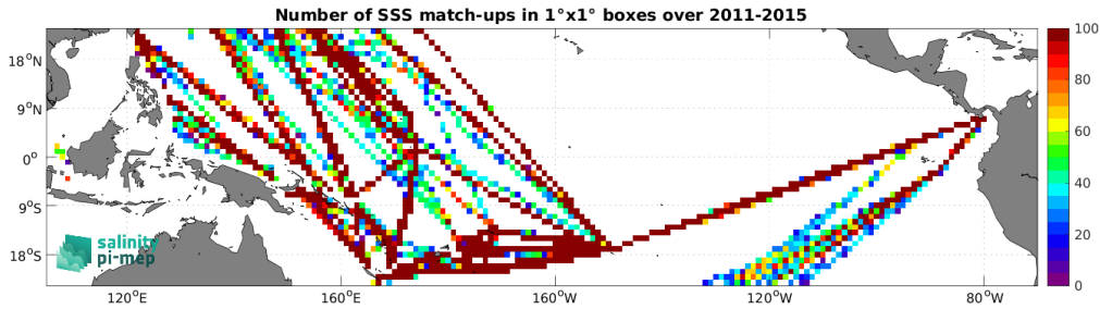
Figure 5: Number of SSS match-ups between TSG (LEGOS-DM) SSS and the Aquarius SSS L3 OR v5 - Monthly (NASA-GSFC) SSS product for the Tropical Pacific Ocean Pi-MEP region over 1^\circ \times 1^\circ boxes and for the full satellite product period.
