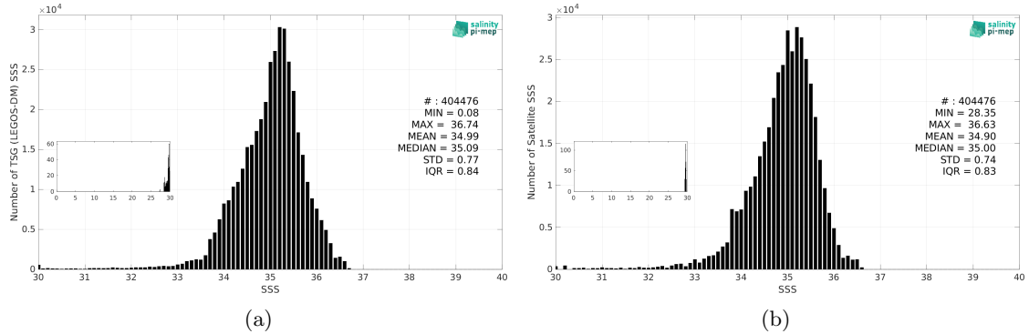
Figure 3: Histograms of SSS from TSG (LEGOS-DM) (a) and Aquarius SSS L3 OR v5 - Monthly (NASA-GSFC) (b) considering all match-up pairs per bins of 0.1 over the Tropical Pacific Ocean Pi-MEP region and for the full satellite product period.
