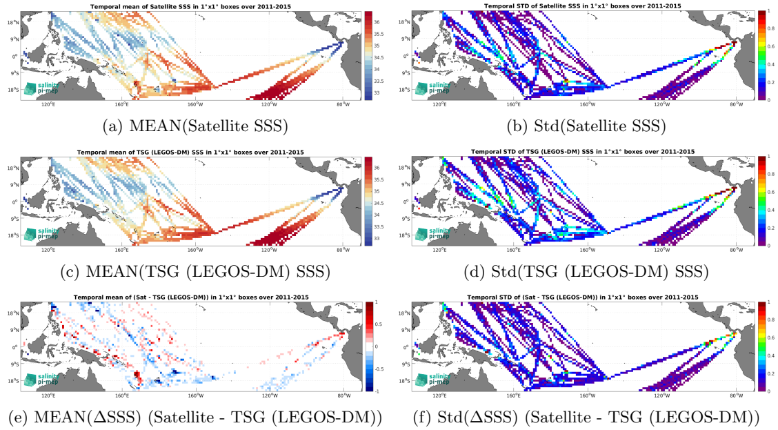
Figure 7: Temporal mean (left) and Std (right) of SSS from Aquarius SSS L3 OR v5 - Monthly (NASA-GSFC) (top), TSG (LEGOS-DM) (middle), and of \Delta SSS (Satellite - TSG (LEGOS-DM)). Only match-up pairs are used to generate these maps.
