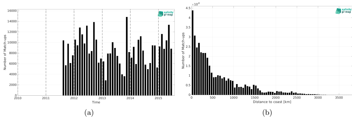
Figure 2: Number of match-ups between TSG (LEGOS-DM) and Aquarius SSS L3 OR v5 - Monthly (NASA-GSFC) SSS as a function of time (a) and as function of the distance to coast (b) over the Tropical Pacific Ocean Pi-MEP region and for the full satellite product period.
