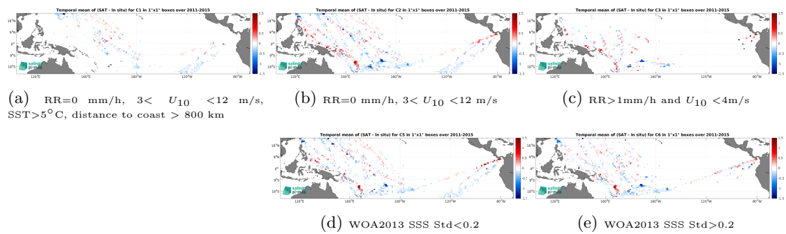
Figure 14: Temporal mean gridded over spatial boxes of size 1^\circ \times 1^\circ of \Delta SSS (Aquarius SSS L3 OR v5 - Monthly (NASA-GSFC) - TSG (LEGOS-DM)) for 5 different subdatasets corresponding to:RR=0 mm/h, 3 < U_{10} < 12 m/s, SST >5^\circ C, distance to coast > 800 km (a), RR=0 mm/h, 3 < U_{10} < 12 m/s (b), RR >1 mm/h and U_{10} < 4 m/s (c), WOA2013 SSS Std <0.2 (d), WOA2013 SSS Std >0.2 (e).
