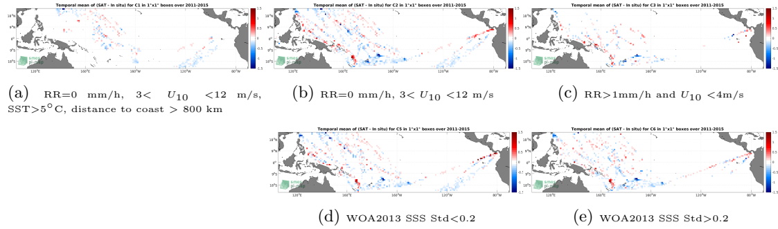
Figure 12: Temporal mean gridded over spatial boxes of size 1^{\circ}\times 1^{\circ} of \Delta\text{SSS} (Aquarius SSS L3 OR v5 - Monthly (NASA-GSFC) - TSG (LEGOS-DM)) for 5 different subdatasets corresponding to:RR=0 mm/h, 3 < U_{10} < 12 m/s, SST >5^{\circ}\text{C} , distance to coast > 800 km (a), RR=0 mm/h, 3 < U_{10} < 12 m/s (b), RR >1 mm/h and U_{10} < 4 m/s (c), WOA2013 SSS Std <0.2 (d), WOA2013 SSS Std >0.2 (e).
