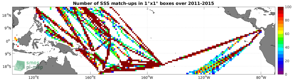
Figure 4: Number of SSS match-ups between TSG (LEGOS-DM) SSS and the Aquarius SSS L3 OR v5 - Monthly (NASA-GSFC) SSS product for the Tropical Pacific Ocean Pi-MEP region over 1^\circ \times 1^\circ boxes and for the full satellite product period.
