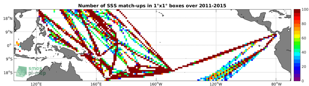
Figure 4: Number of SSS match-ups between TSG-LEGOS-DM SSS and the Aquarius-L3-OR-V5-MONTHLY-1DEG SSS product for the Tropical Pacific Ocean Pi-MEP region over 1^\circ \times 1^\circ boxes and for the full satellite product period.
