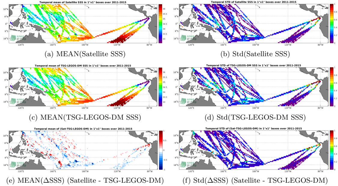
Figure 6: Temporal mean (left) and Std (right) of SSS from Aquarius-L3-OR-V5-MONTHLY-1DEG (top), TSG-LEGOS-DM (middle), and of \Delta SSS (Satellite - TSG-LEGOS-DM). Only match-up pairs are used to generate these maps.
