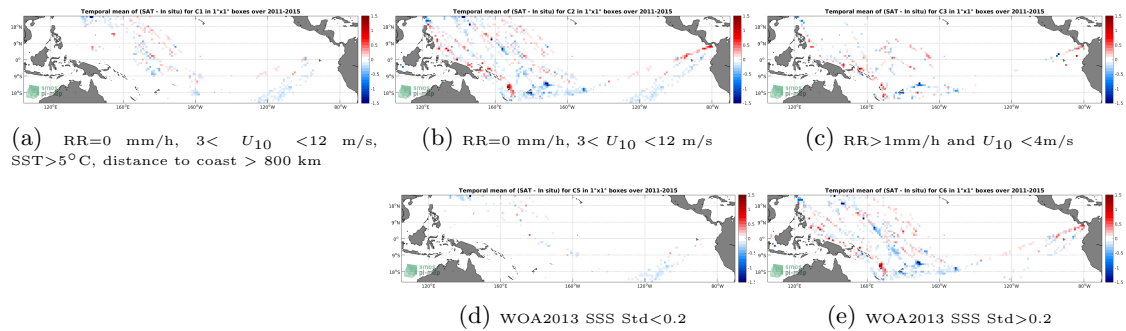
Figure 12: Temporal mean gridded over spatial boxes of size 1^\circ \times 1^\circ of \Delta SSS (Aquarius-L3-OR-V5-MONTHLY-1DEG - TSG-LEGOS-DM) for 5 different subdatasets corresponding to:RR=0 mm/h, 3 < U_{10} < 12 m/s, SST > 5^\circ\text{C} , distance to coast > 800 km (a), RR=0 mm/h, 3 < U_{10} < 12 m/s (b), RR > 1 mm/h and U_{10} < 4 m/s (c), WOA2013 SSS Std < 0.2 (d), WOA2013 SSS Std > 0.2 (e).
