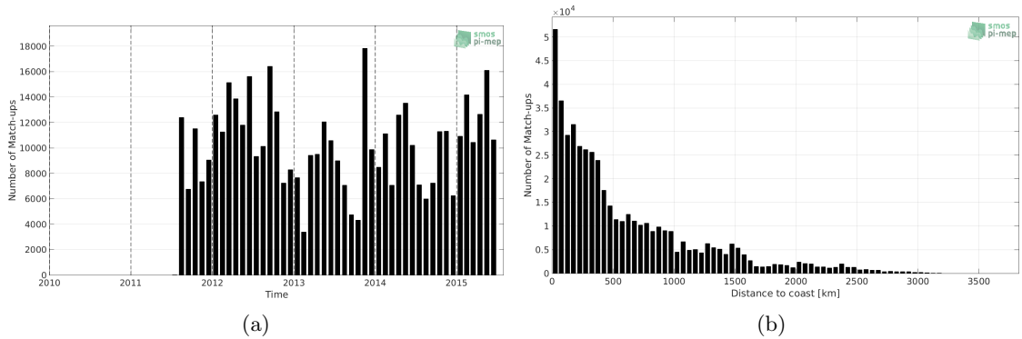
Figure 1: Number of match-ups between TSG-LEGOS-DM and Aquarius-L3-OR-V5-MONTHLY-1DEG SSS as a function of time (a) and as function of the distance to coast (b) over the Tropical Pacific Ocean Pi-MEP region and for the full satellite product period.
