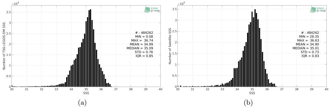
Figure 2: Histograms of SSS from TSG-LEGOS-DM (a) and Aquarius-L3-OR-V5-MONTHLY-1DEG (b) considering all match-up pairs per bins of 0.1 over the Tropical Pacific Ocean Pi-MEP region and for the full satellite product period.
